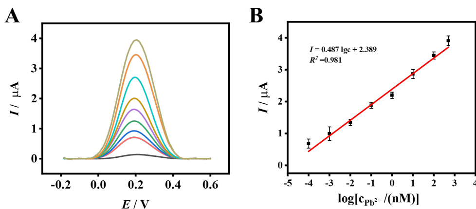
Fig. 5. (A) SWV responses of constructed DNA biosensor to different concentrations of \text{Pb}^{2+} (from a to i: 0, 0.1 pM, 1 pM, 10 pM, 100 pM, 1 nM, 10 nM, 100 nM, and 500 nM). (B) Calibration plot of SWV peak current versus the logarithm of \text{Pb}^{2+} concentration.
