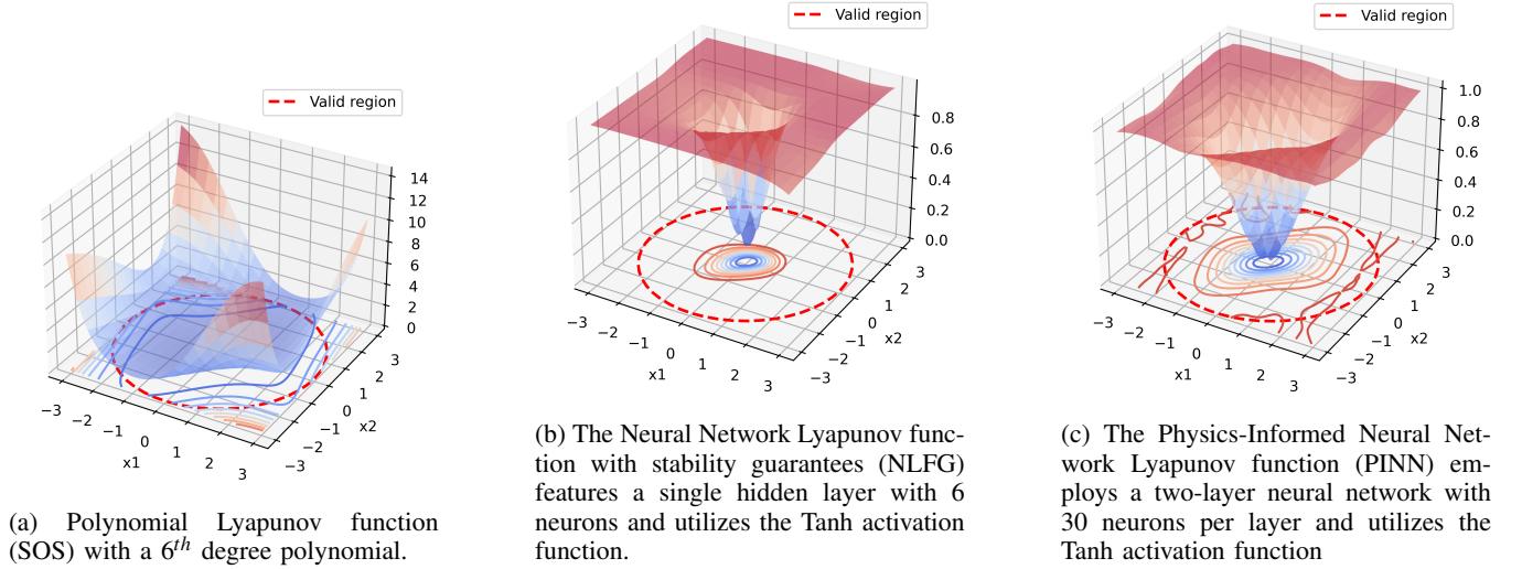
Fig. 1: Experimental Results for the Van der Pol system ( \mu = 1 ).
