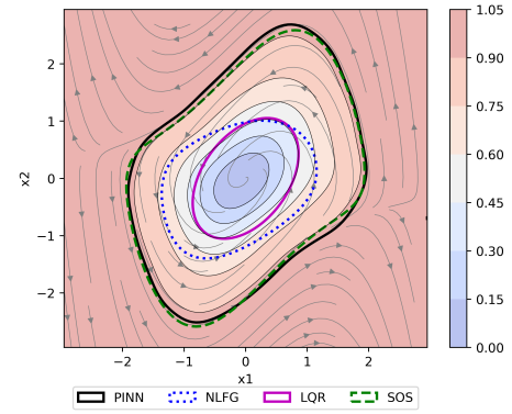
Fig. 2: Comparison of the Regions of Attraction (ROA) for Quadratic (LQR), Sum-of-Squares (SOS), Neural Lyapunov Function with stability guarantees (NLFG), and Physics-informed Neural Lyapunov Function (PINN) methods
