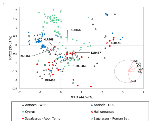
Fig. 13 Principal Component analysis (PCA). Multivariate analysis of seven oxides ( \text{Na}_2\text{O} , \text{MgO} , \text{Al}_2\text{O}_3 , \text{SiO}_2 , \text{K}_2\text{O} , \text{CaO} , and \text{TiO}_2 ) using the compositions of the samples from the House of Charidemos, Antioch [21], Cyprus [22], and Sagalassos [18]
