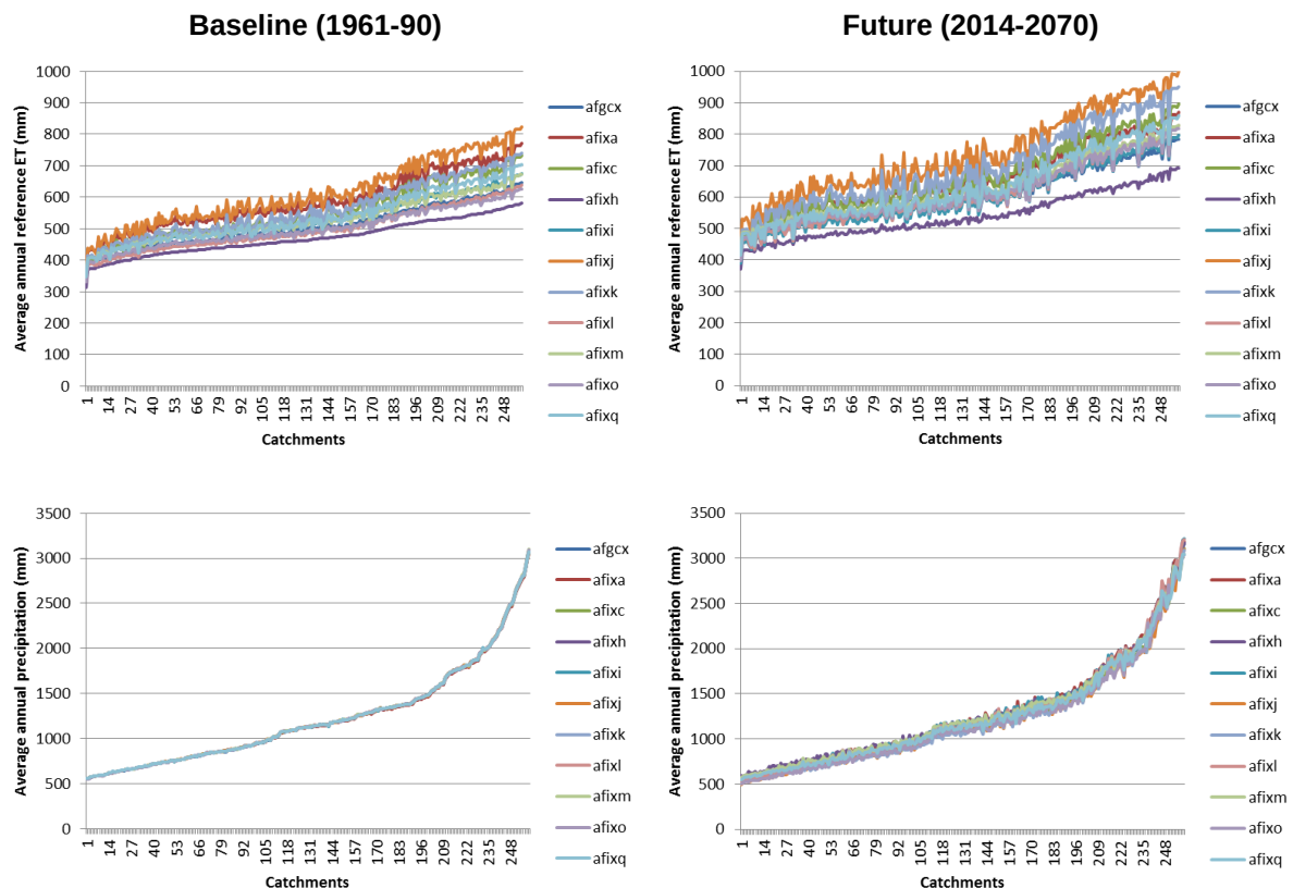
Figure 2.6 Comparison of the baseline and future average annual reference evapotranspiration and precipitation for FutureFlows ensemble members (ranked according to baseline afixh values)
