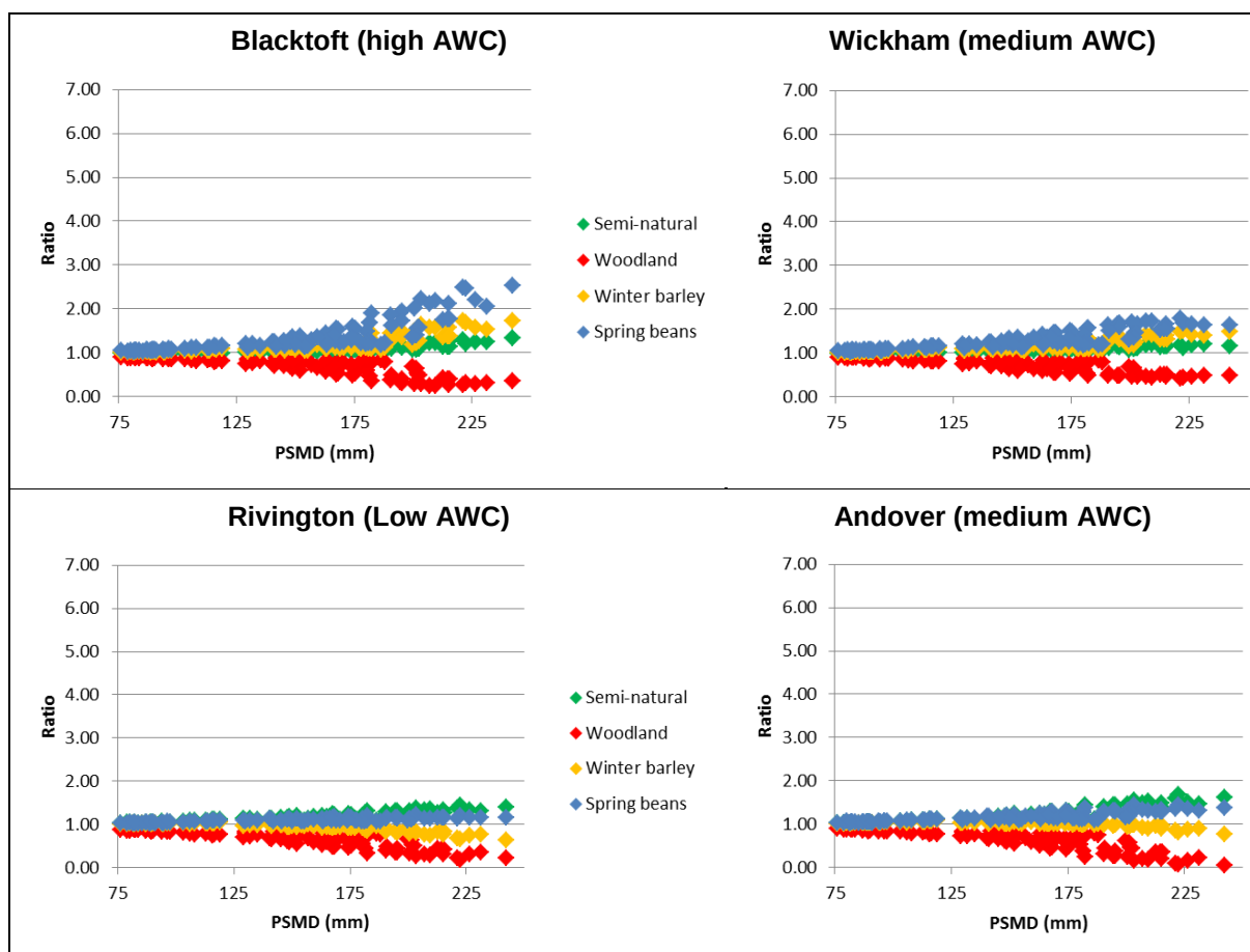
Figure 3.1 Changes in baseline average annual Hydrologically Effective Rainfall (AAHER) under different vegetation types, expressed as a ratio of the AAHER under permanent grassland (a value of 1 indicates no difference)
