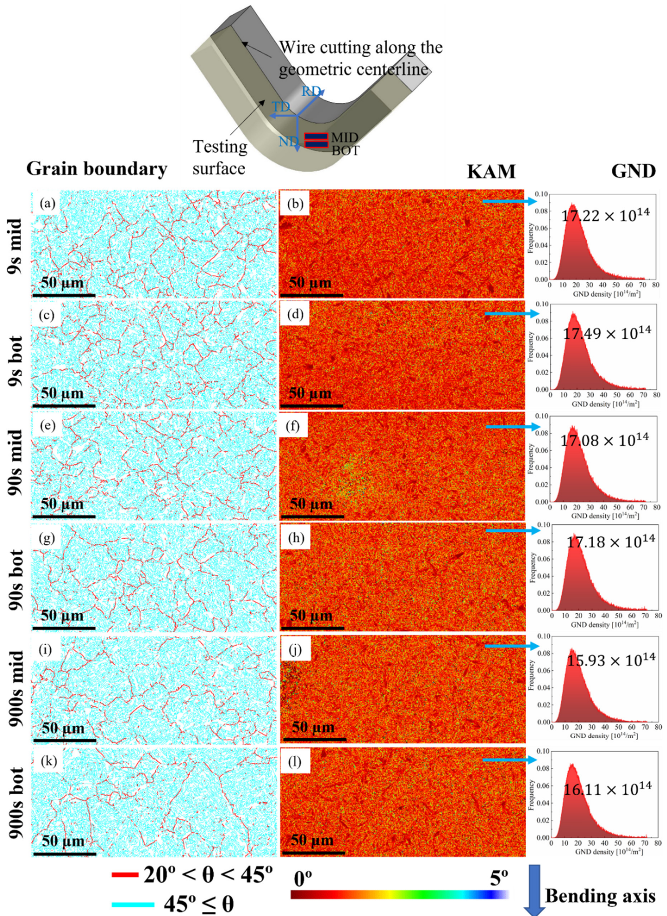
Figure 2. (a,c,e,g,i,k) GB maps under different bending rates in the mid and bot areas; (b,d,f,h,j,l) corresponding KAM maps and GND density distribution.
