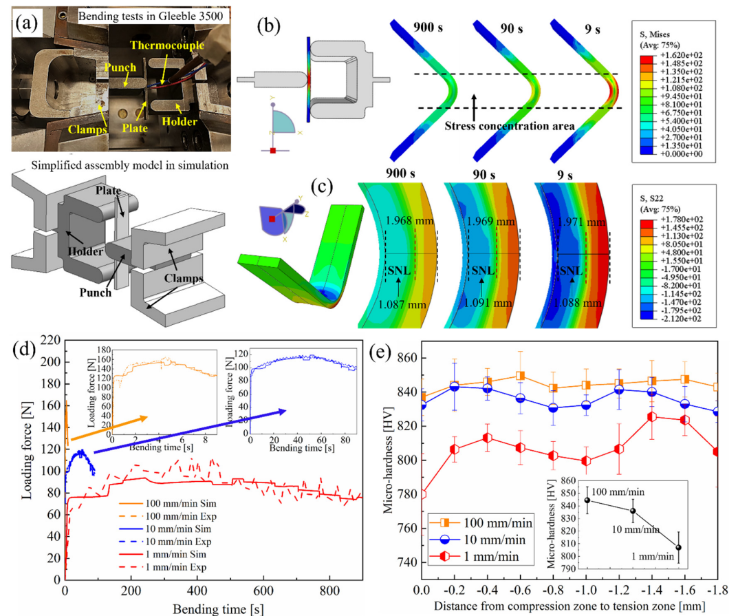
Figure 1. (a) Diagrammatic drawing of the simplified model; (b) equivalent stress distribution; (c) transverse stress (S22) distribution; (d) the comparison of simulated loading force with experiments; and (e) hardness distribution under different bending conditions.
