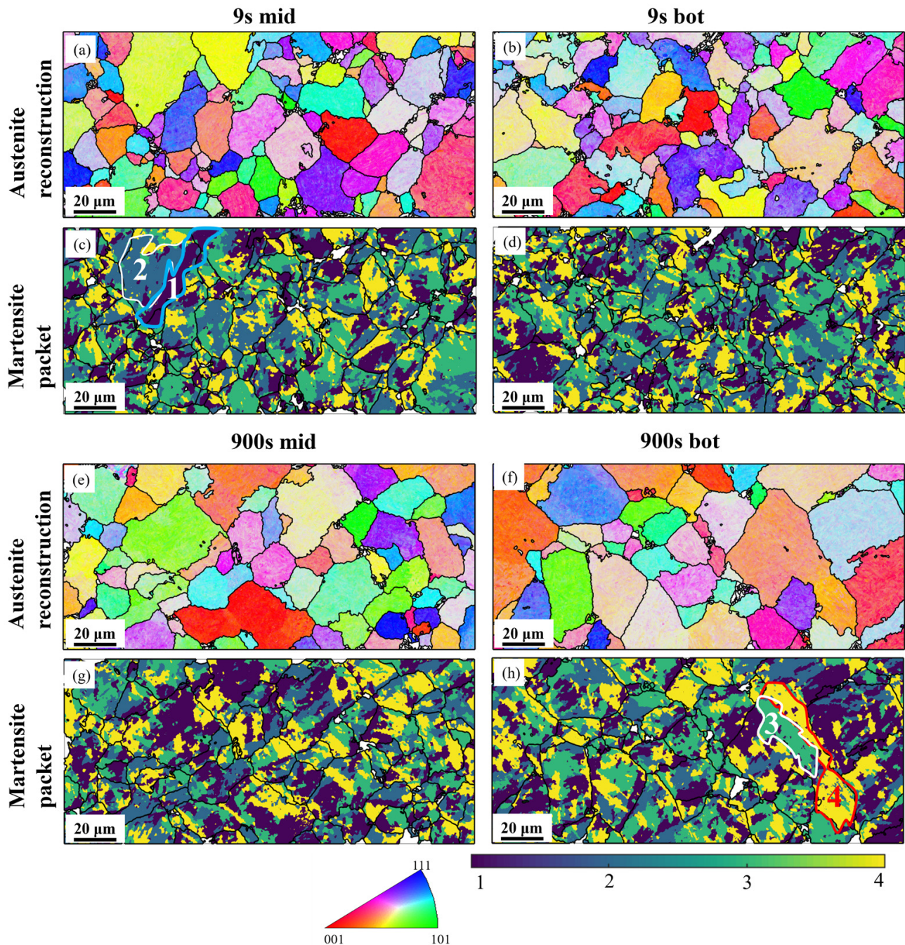
Figure 3. (a,b,e,f) Parent austenite grain reconstruction of different bent samples at mid and bot areas; (c,d,g,h) corresponding distribution of martensite packet.
