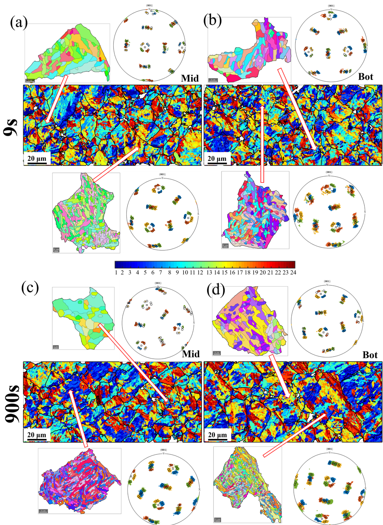
Figure 4. Martensite variants of samples bent at 100 mm/min of (a) mid and (b) bot areas and 1 mm/min of (c) mid and (d) bot areas; the individual grain and corresponding pole figures are provided.
