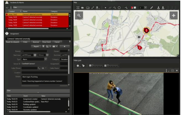
Fig. 11: SAFE user-interface during inference of the model
