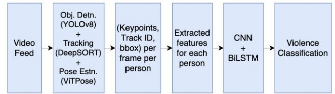
Fig. 1: Architecture of the proposed violence detection framework
