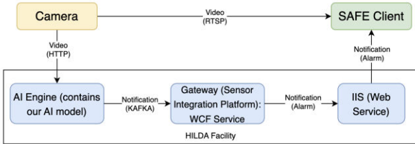
Fig. 6: System Architecture
