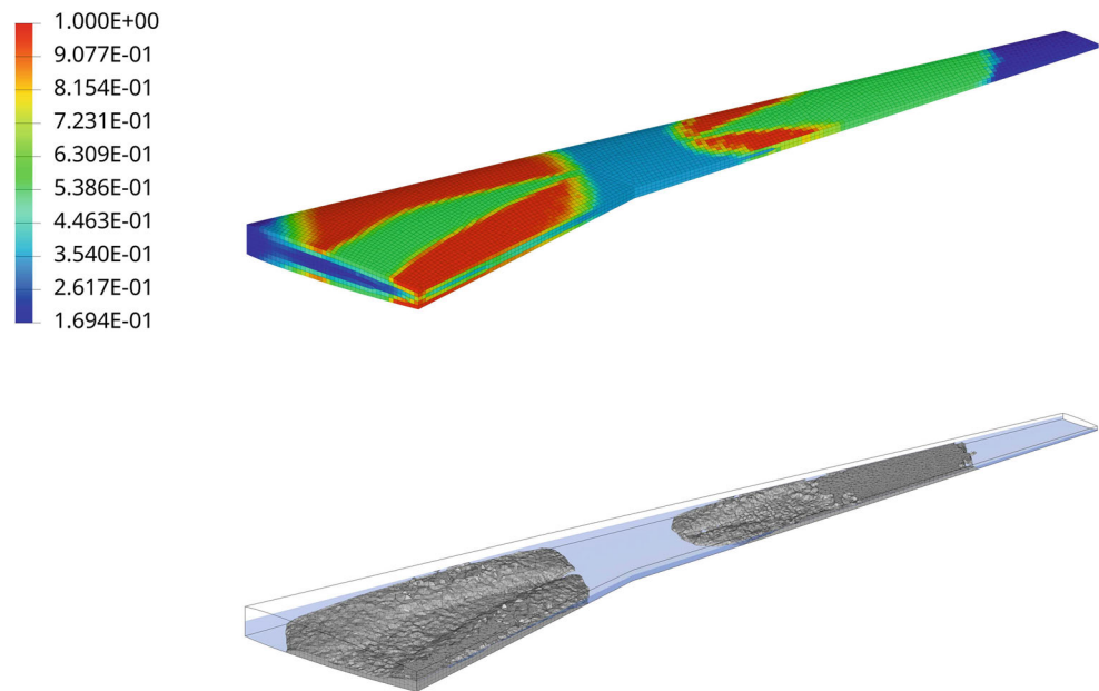
Fig. 12 Density contour plot corresponding to a local optimum for frequency maximisation (top). Cut along the span (bottom). Only densities \rho \geq 0.5 are visualised to highlight the main features
