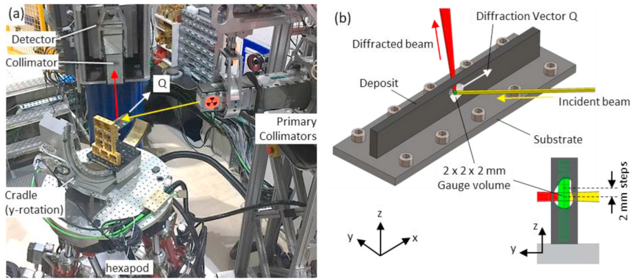
Fig. 1. a) setup of specimen on SALSA; b) location of gauge volumes and hardness plot line.
