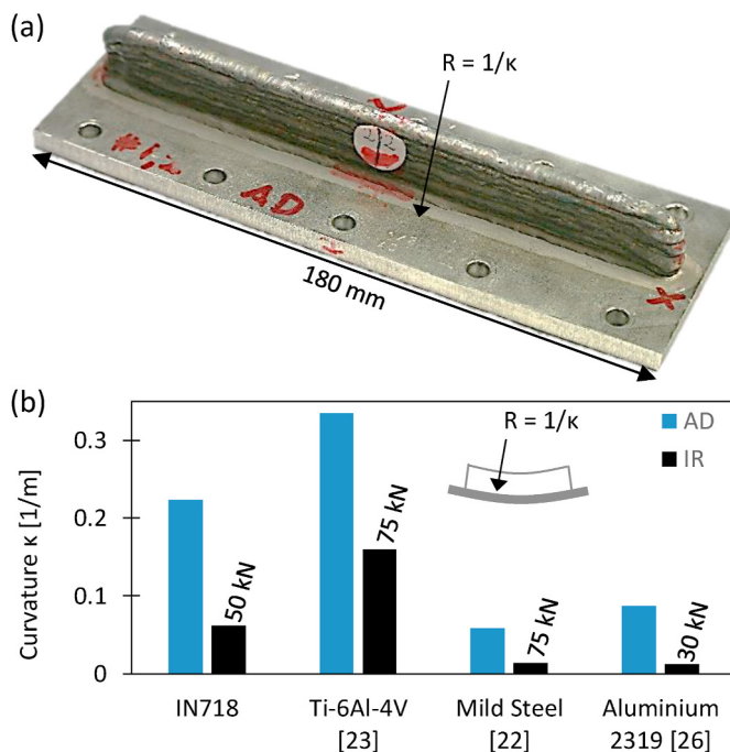
Fig. 3. Curvature of the distorted substrate after depositing 4 structural metals with WAAM with the same cross-sectional geometry [22,23,26].
