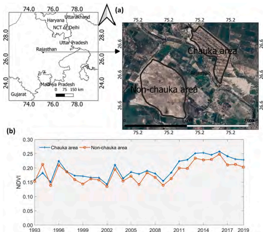
Fig. 12. Location of Chauka and non- Chauka areas (panels (a)), and NDVI from 1993 to 2019 in Chauka and non- Chauka areas (panel (b)).
