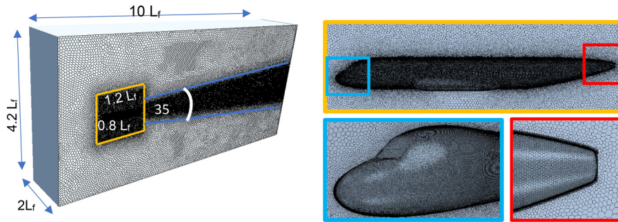
Figure 2 A320 Neo domain mesh generation strategy that is also used for the optimisation simulations showing the refinement regions on the fuselage
