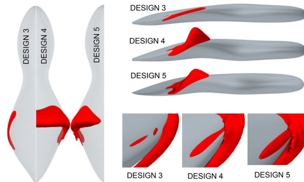
Figure 7 The boundary where flow has Mach > 1 in a 3D domain on the optimised Designs 3–5
