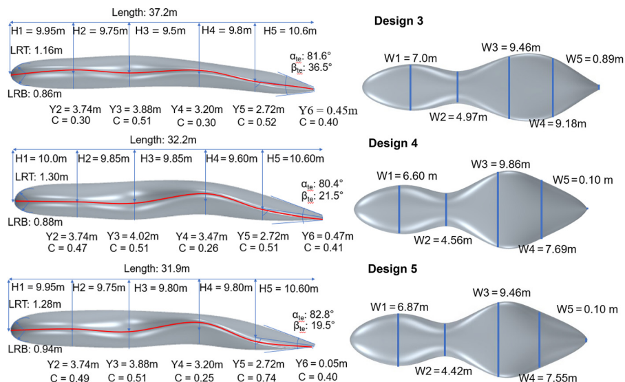
Figure 3 Designs 3–5 fuselage geometry comparison using its constructed parameters
