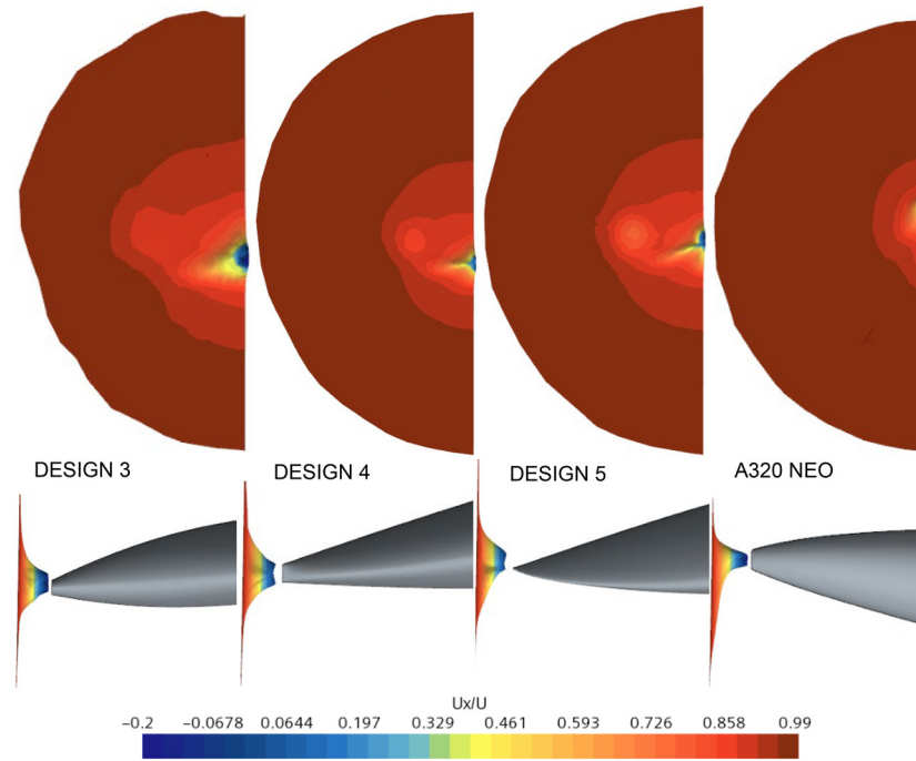
Figure 6 3D volume relative velocity U_x/U_\infty contouring on front and side view for fuselage Designs 3–5 and A320 Neo
