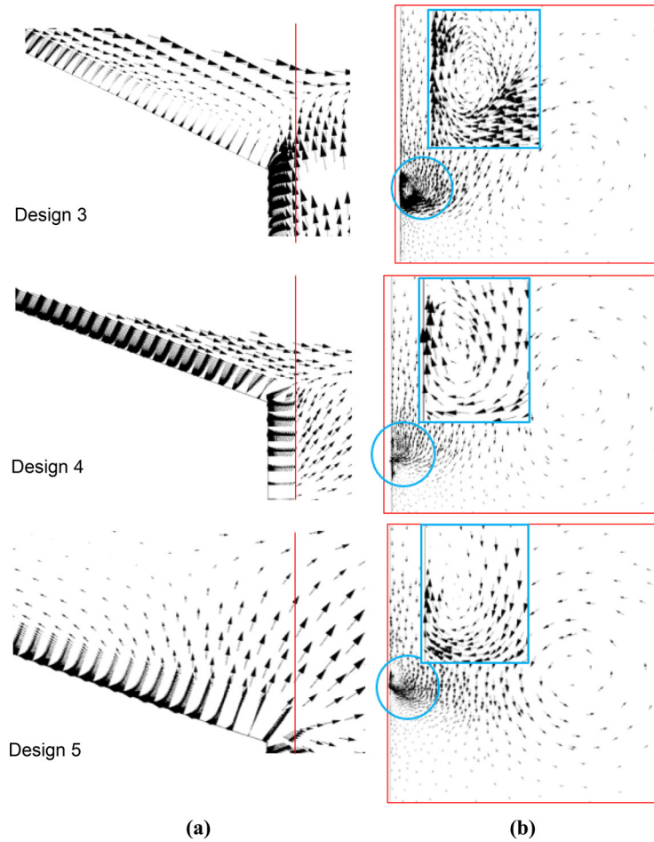
Figure 5 Streamwise velocity vector glyphs for Designs 3–5 are shown on the left-hand side. Transverse velocity vector glyphs for Designs 3–5 are shown on the right-hand side which correlates with the red line location on the left-hand side. The blue box is an enlargement of the vortex at the centreline of the fuselage
