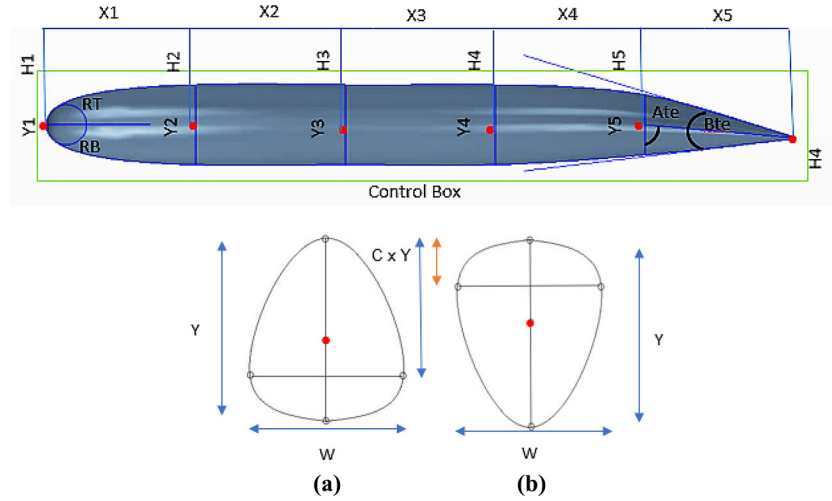
Figure 1 Parameterisation of the fuselage in the longitudinal direction and cross-section of the fuselage showcasing a bottom-heavy oval and a top-heavy oval fuselage cross-section
