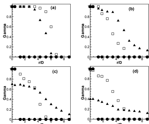
Fig. 19 Radial profiles of scalar intermittency at (a) x=40\text{mm} , (b) x=80\text{mm} , (c) x=100\text{mm} and (d) x=120\text{mm} . Here, circles denote jet results, squares denote bluff body stabilised jet results and triangles denote body stabilised swirl jet results.
