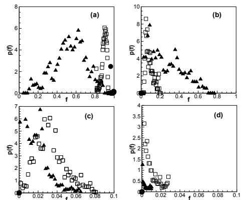
Fig. 17 Probability density function (pdf) of the passive at x=40\text{mm} . Here, circles, squares and triangles indicate results for the jet, bluff body stabilised jet and bluff body stabilised swirl jet, respectively.
