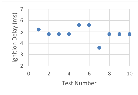
Fig. 17. Ground mix ignition delay at 40 W and 1.0 mm beam width.
