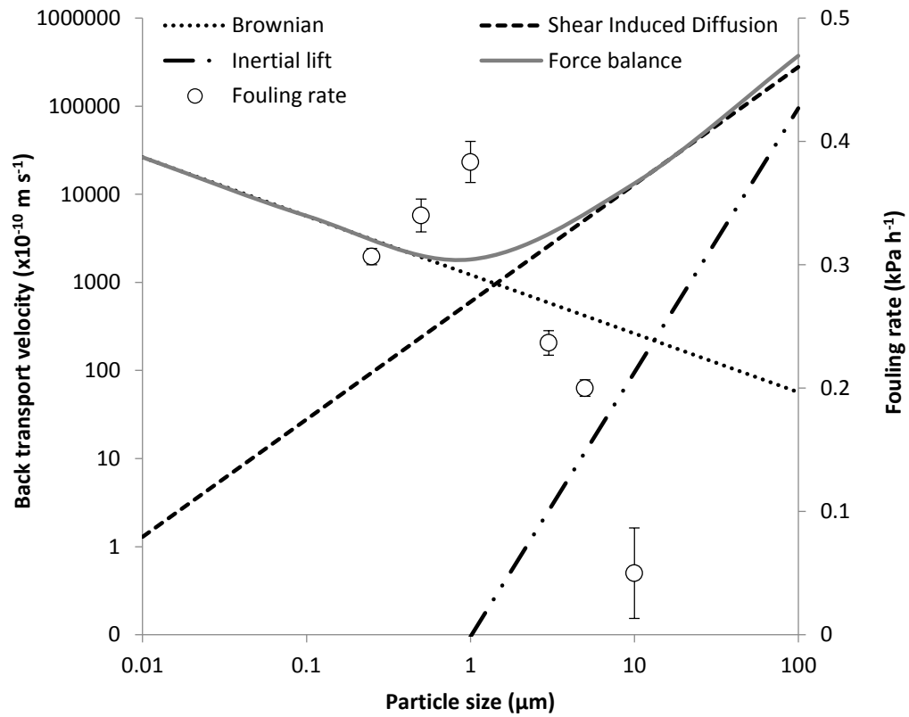
Figure 3. Fouling rate determined for particle mono-dispersions and compared to modelled back-transport velocities (0.25 to 10 \mu\text{m} ). C_b 0.01 \text{kg m}^{-3} ; V_L 0.011 \text{m s}^{-1} .
