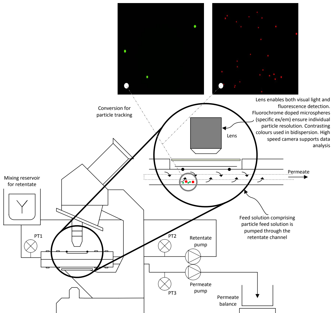
Figure 2. Experimental set-up.
