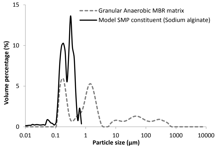
Figure 1. Particle size distribution of an anaerobic MBR used to evidence bimodal distribution, with a peak in the sub-micron range. This is compared the model polysaccharide Sodium Alginate, often used as a surrogate of SMP, whose particle size is within the sub-micron range.
