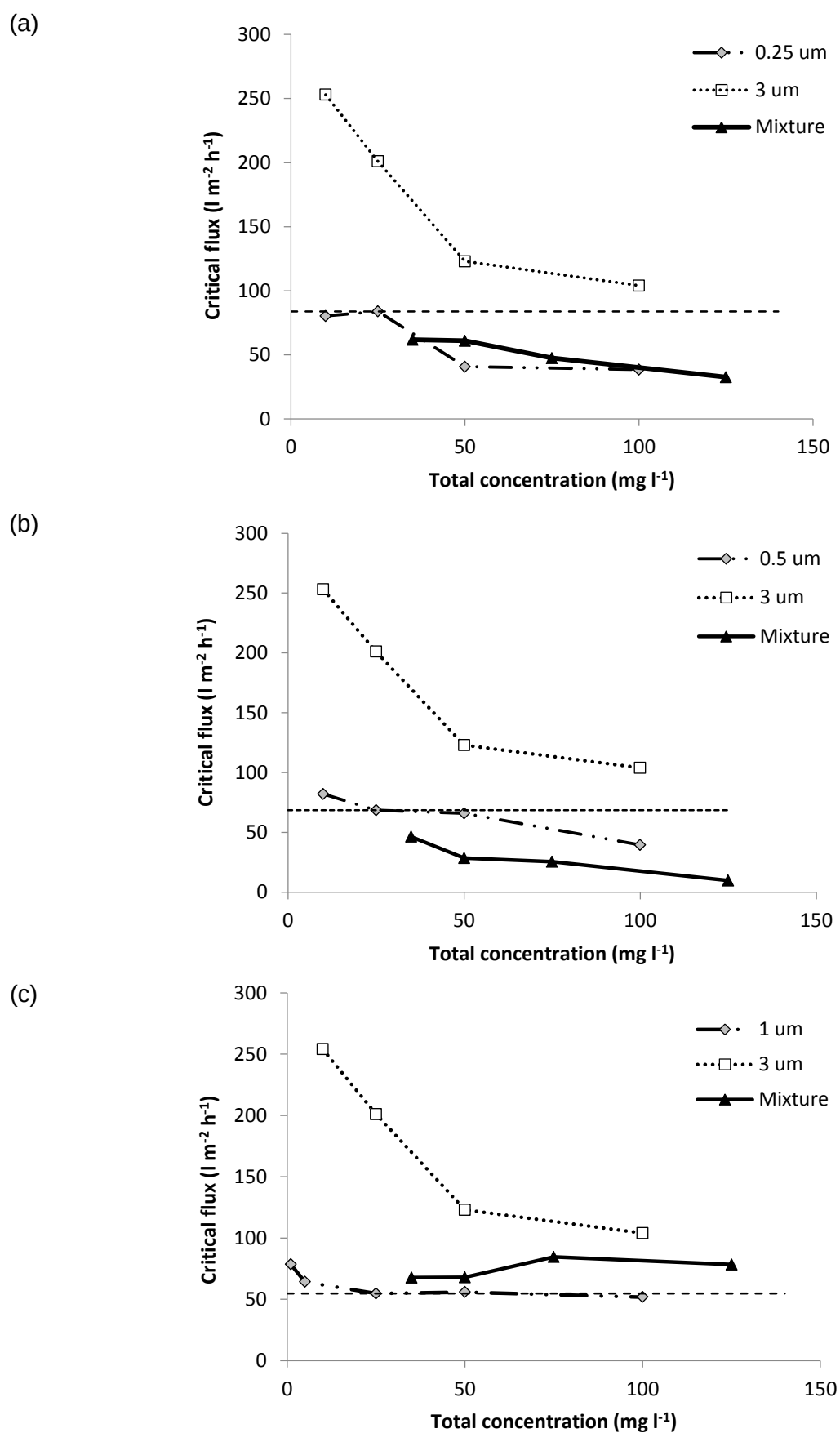
Figure 5. Critical flux ( J_c ) determination for mono-dispersions and binary dispersions using the flux-step method. C_b 0.01 \text{ kg m}^{-3} ; V_L 0.011 \text{ m s}^{-1} .
