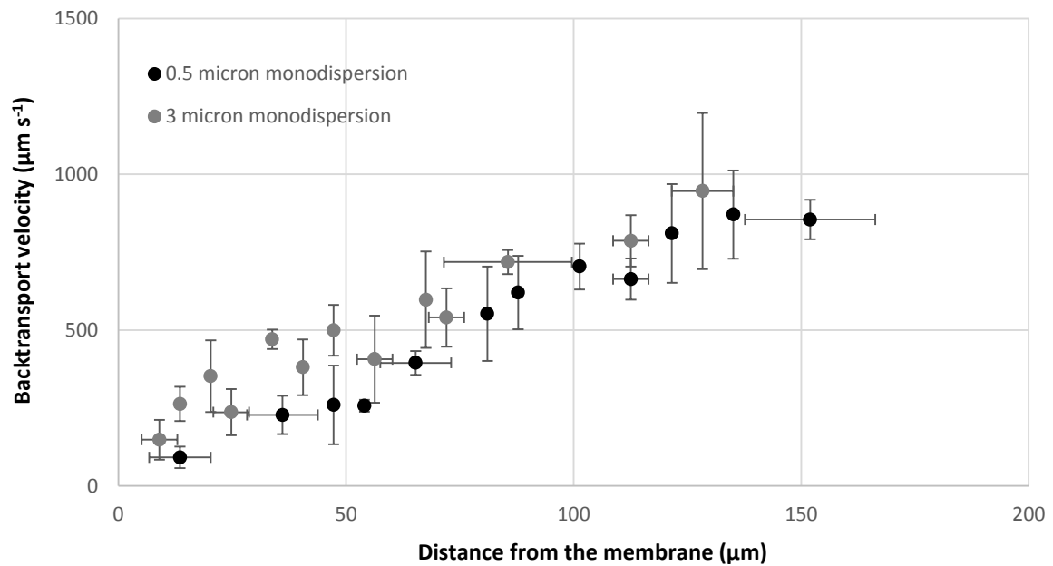
Figure 4. Measured particle back-transport velocities ( \mu\text{m s}^{-1} ) for particle mono-dispersions in the polarised region adjacent to the membrane. C_b 0.01 \text{kg m}^{-3} ; V_L 0.011 \text{m s}^{-1} .
