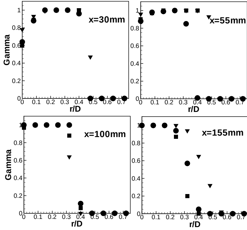
Figure 19: Radial profiles of temperature intermittency at (a) x=30\text{mm} , (b) x=55\text{mm} , (c) x=100\text{mm} and (d) x=155\text{mm} . Here circles, squares and inverted triangles denote results for swirl numbers 0.5, 0.75 and 1.0
