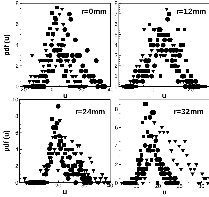
Figure 8: Comparisons of velocity pdfs at x=155\text{mm} at equidistant radial locations (a), (b), (c) and (d). Here circles, squares and inverted triangles denote results for swirl numbers 0.5, 0.75 and 1.0
