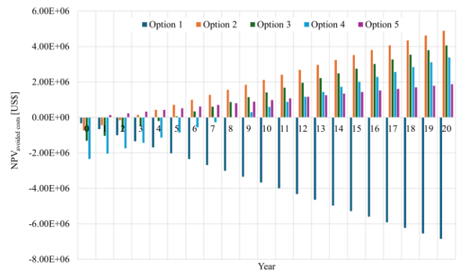
Fig. 2. Cumulated NPV_{\text{avoided cost}} for proposed configurations
