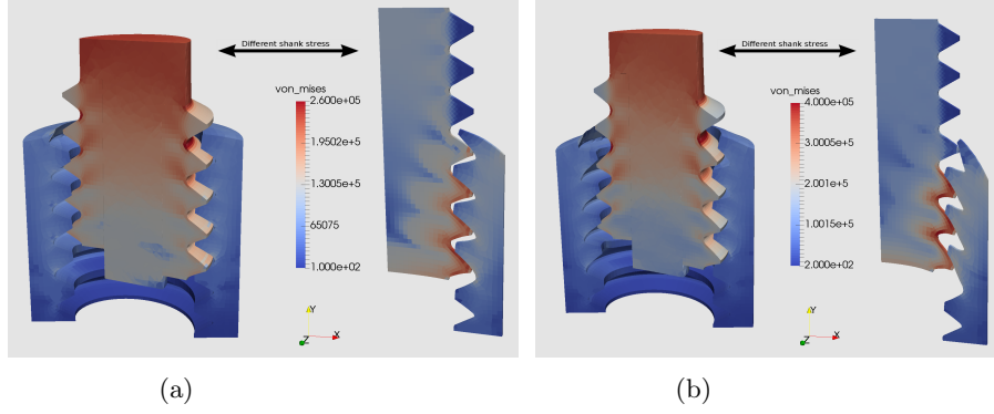
Figure 11: von Mises stress fields for 2.5D and 3D models at 30% (Left) and 70% (Right) of the maximum applied displacement.
