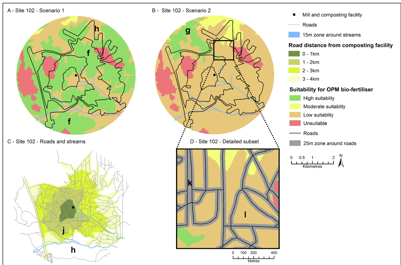
Fig. 4. Application of tool to KKP 102 Bukit Leelau, Pahang. (A) and (B) Land suitability for biofertiliser application in Scenarios 1 and 2. (C) Roads, road travel distance zones, streams, streambank 15 m buffer zones. (D) Zoom-in detail with 25 m roadside zones.
