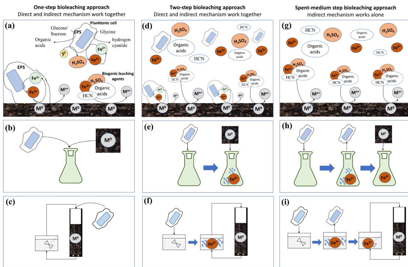
Fig. 3 Bioleaching approaches used for metal solubilisation a mechanism of the one-step bioleaching approach; in this approach, both microorganisms and metal-bearing material are added to the medium at the same time, and the bioleaching process is carried out during the microorganisms culturing b one-step approach in shake flask, c one-step approach in column, d mechanism of the two-step bioleaching approach; in this approach, first, the microorganisms are cultivated in the absence of solid waste, then after microorganisms are reached the log phase, metal-bearing material is added into the culture to start the bioleaching, e two-step approach in shake flask, f two-step approach
