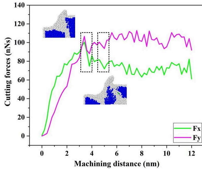
(a) Scratch forces during cutting of a polycrystalline GaAs
