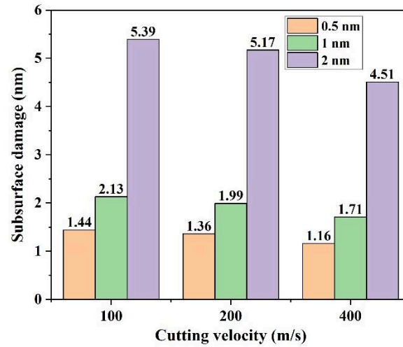
288 Fig. 10. Sub-surface damage depth at different cutting velocities and depth of cut
