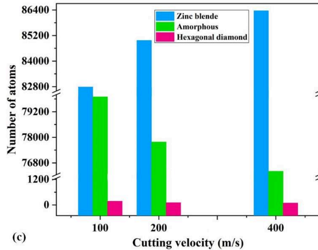
Fig. 4. The evolution of microstructure changes in polycrystalline GaAs during nanoscratching process with various cutting velocities under cutting depth of 0.5 nm (a), 1 nm (b) and 2 nm (c). Note here that the occurrence of the formation of hexagonal diamond is a mere artefact since the potential function used in this study does not distinguish energy differences between cubic and hexagonal phases.
