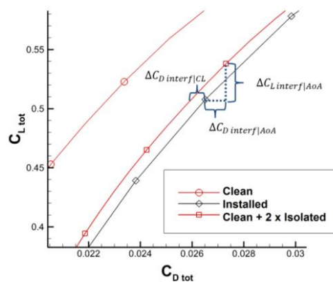
Fig. 9 Definition of interference terms on the typical lift-drag polars for clean wing, clean wing with isolated engine and wing-installed engine
