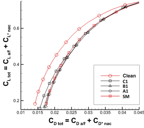
Fig. 14 Lift-drag polar for CRM aircraft without (Clean) and with engines (C1/B1/A1), compared with drag polar created as superposition (SM) of clean wing and isolated engines data (SM); Re = 45 \times 10^6 ; M = 0.82 ;
