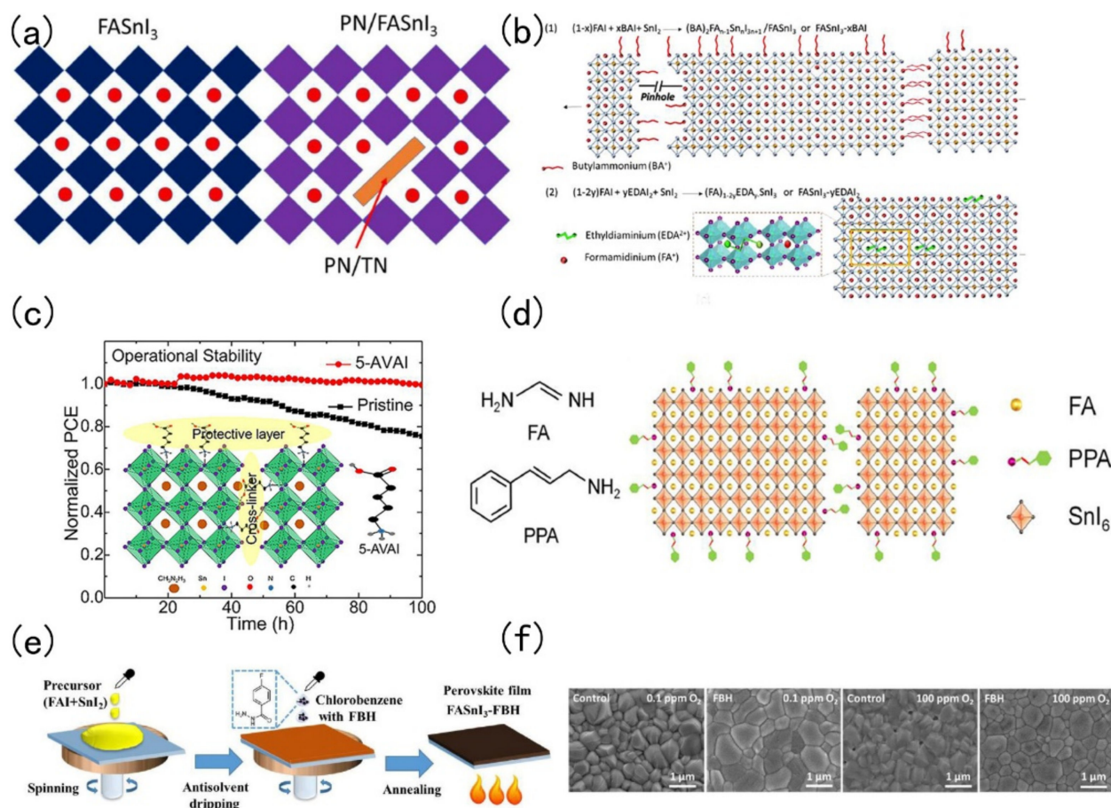
Figure 2. (a) Internal structure of PN/TN acting on perovskite). Reproduced with permission from [38]. Copyright 2016 American Chemical Society. (b) Internal structure of \text{BA}^+/\text{EDA}^+ acting on perovskite. Reproduced with permission from [44]. Copyright 2018 The Royal Society of Chemistry. (c) The stability of the device with 5-AVAI modification over time and the stability of the device without 5-AVAI modification with time (inside is the diagram of the internal structure of 5-AVAI acting on perovskite). Reproduced with permission from [45]. Copyright 2019 American Chemical Society. (d) The chemical structure formula of FA/PPA and the internal structure of PPA acting on perovskite. Reproduced with permission from [46]. Copyright 2019 Elsevier Inc. (e) Flow chart of FBH modified perovskite films. Reproduced with permission from [48] Copyright 2020 The Royal Society of Chemistry. (f) Scanning electron microscopy image of perovskite film made with/without FBH under different oxygen conditions. Reproduced with permission from [48] Copyright 2020 The Royal Society of Chemistry.
