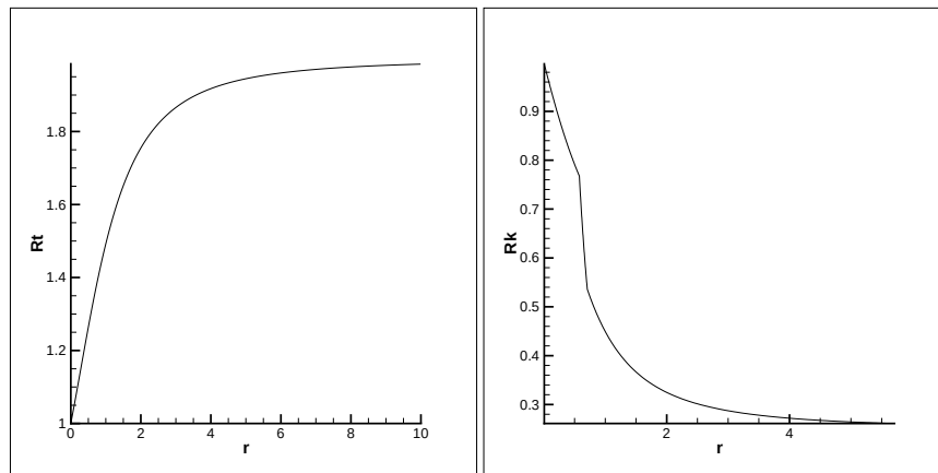
(a) Ratio of spectral radii (Eq. 34) (b) Ratio of characteristic condition number (Eq. 35)
