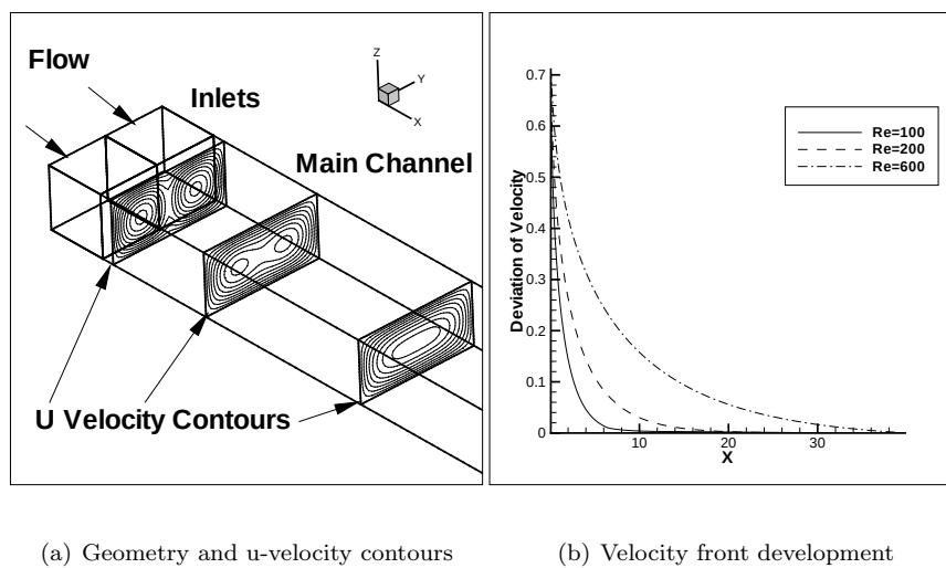
Figure 6. Three-dimensional flow in a channel with two inlets
