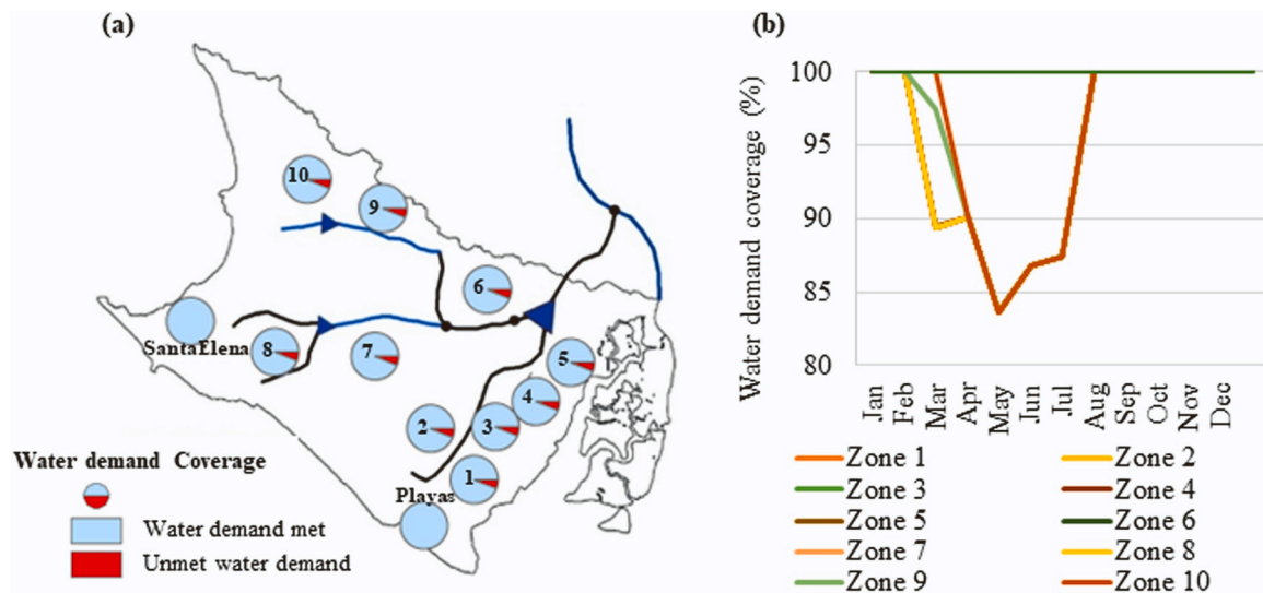
Fig. 5. Simulated annual average water demand coverage (spatial analysis) (a) and monthly average water demand coverage (temporal analysis) for each irrigation zone and urban demand site (b).
