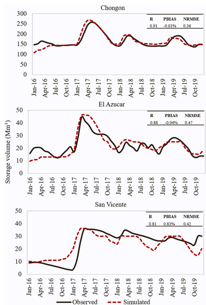
Fig. 3. Comparison of WEAP simulated (dotted line) and observed (solid line) monthly reservoir storage volumes (Mm 3 ) for each reservoir in the SEP.
