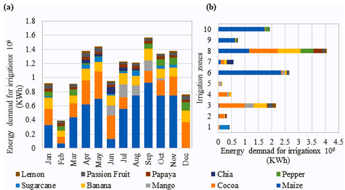
Fig. 7. Simulated average monthly energy consumption by crop type (a) and annual average energy consumption (kWh) for each irrigation zone (b).
