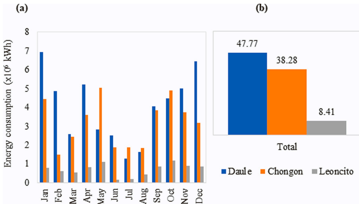
Fig. 6. Simulated monthly variation in energy consumption (left panel) and annual energy use at each pumping station (right panel) in million kWh.
