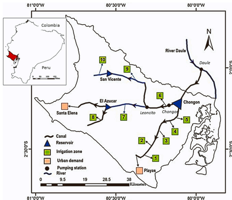
Fig. 1. Schematic representation of water infrastructure including reservoirs, irrigation zones, pumping stations and urban water demand sites across the Santa Elena Peninsula (based on CEDEGE (2001)).
