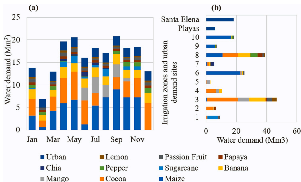
Fig. 4. Simulated monthly average irrigation water demand (Mm³) by crop (a) and annual average water demand for each irrigation zone, by crop type including urban demand (b).
