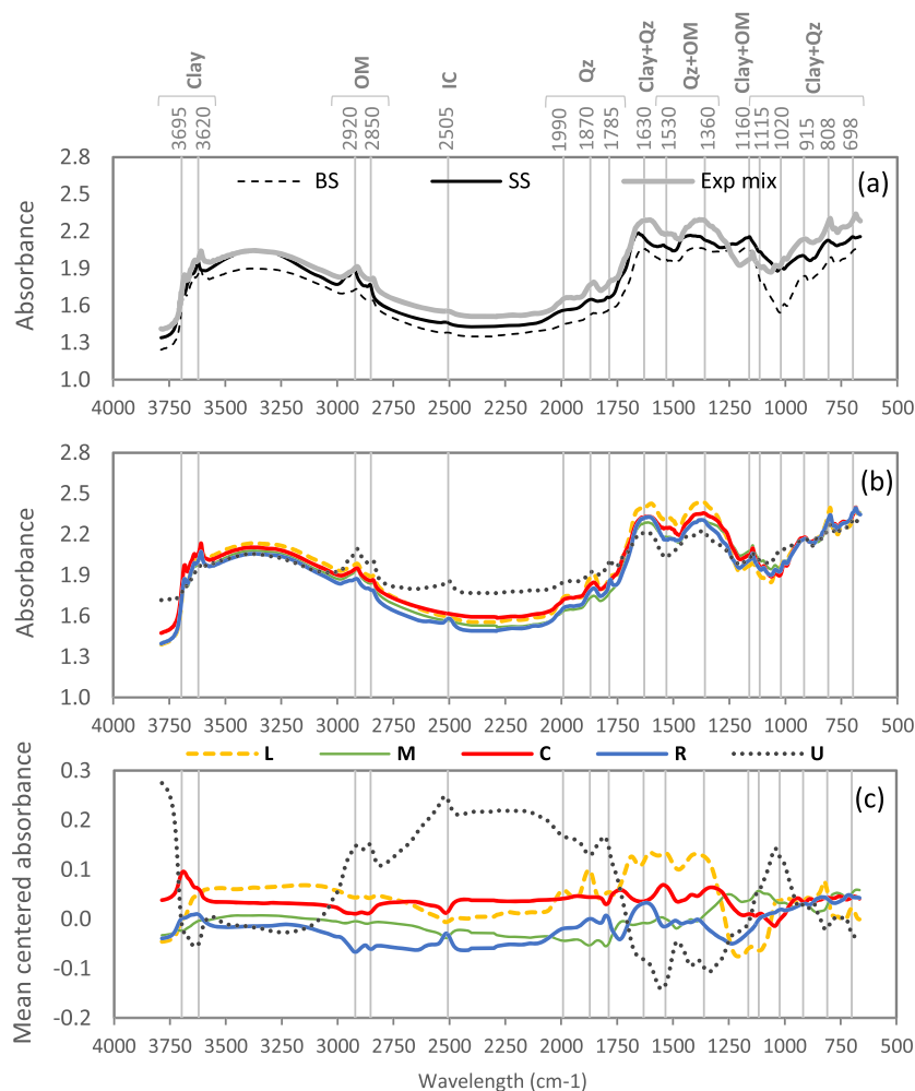
FIGURE 3 Mean diffuse reflectance infrared Fourier transform spectrometry spectra of (a) suspended sediment (SS), bed sediment (BS), and experimental mixtures (Exp. mix); (b) unprocessed and (c) preprocessed (i.e., smoothed and mean centred) sediment source samples. Vertical lines represent absorption peaks ascribed to clay minerals, organic matter (OM), inorganic carbon (IC), and quartz (Qz)
