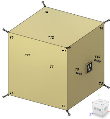
Figure 6: Spacecraft basic physical model with thruster positions labelled
