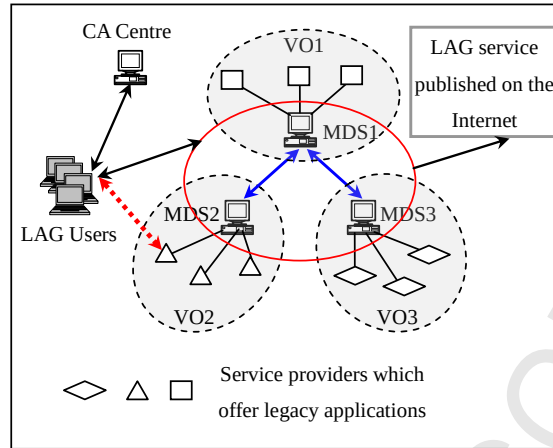
Fig.1. Architecture of the legacy application grid
