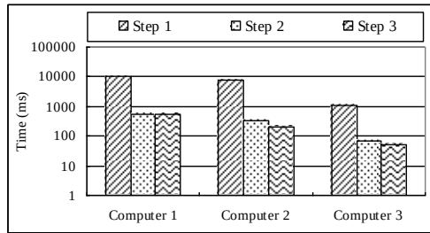
Fig.4 Average registration overhead
