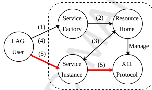
Fig.3 Components and workflow of the legacy service
