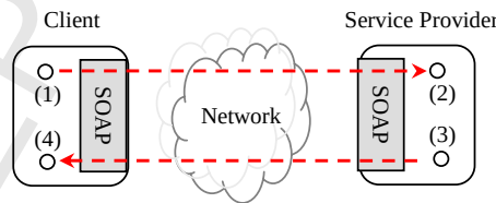
Fig.6 Test scenario of a grid service invocation
