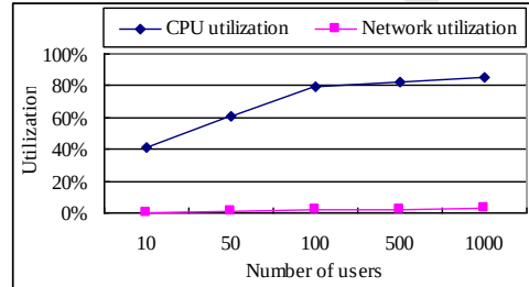
Fig.8 CPU and network utilization
