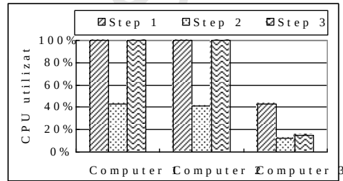
Fig.5 CPU utilization
