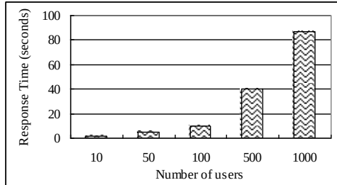
Fig.7 Average query time
