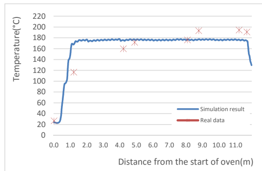
Fig. 10. Comparison of the product temperature between simulation result and experimental data.
