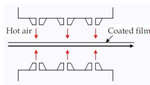
Fig. 1. Typical diagram of convection oven with impinging hot air jets.
