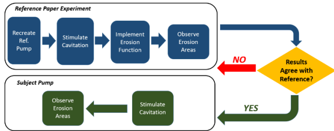
FIGURE 2: SEQUENCE OF STEPS TO PREDICT EROSION USING CFD AND APPLICATION TO SUBJECT PUMP
