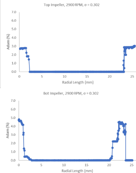
FIGURE 11: WEAR DISTRIBUTION ACROSS SUBJECT PUMP AT 2900 RPM
