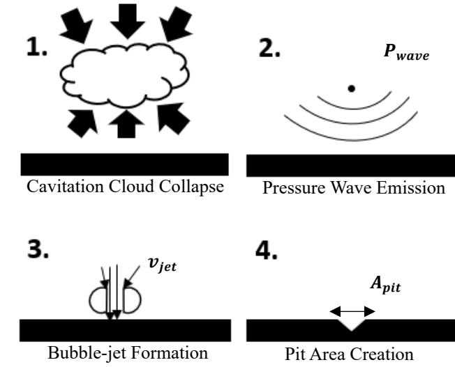
FIGURE 1: EVENTS RELATED TO CAVITATION DAMAGE
