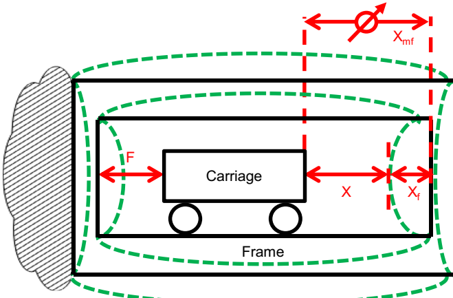
Fig. 2. Motion system 2D model of a flexible frame.
