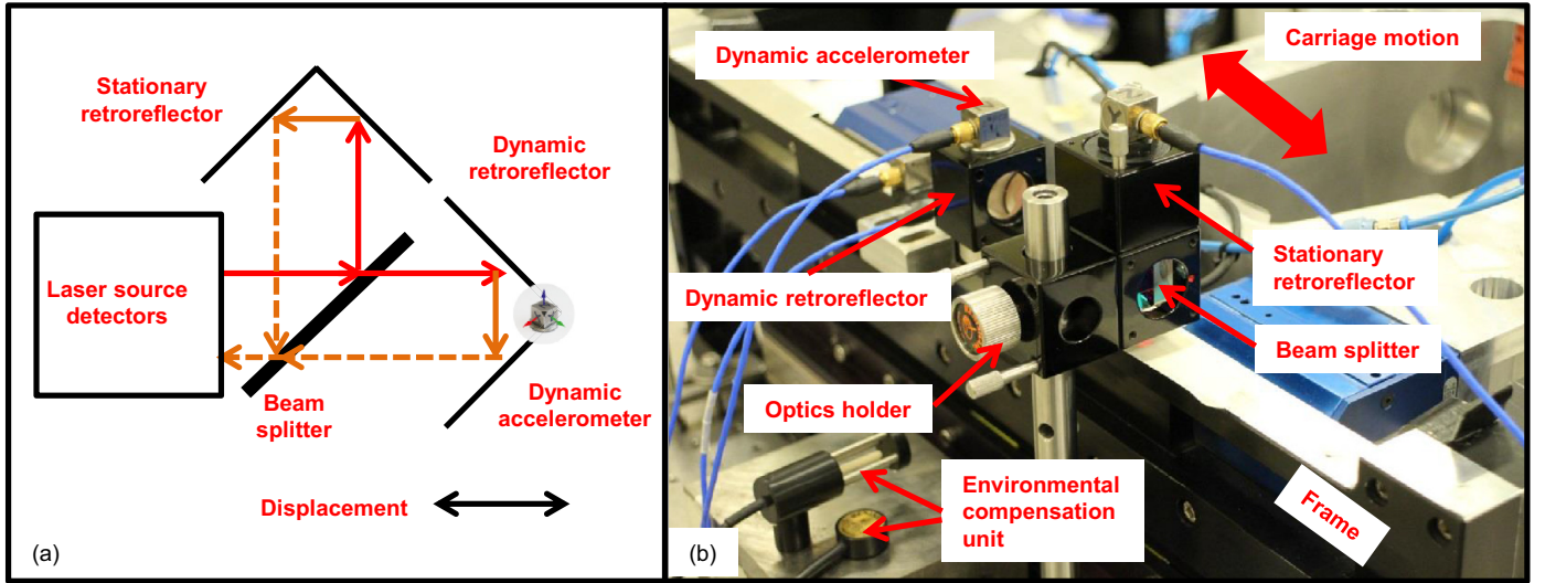
Fig. 8. Setup of the displacement validation experiment.
