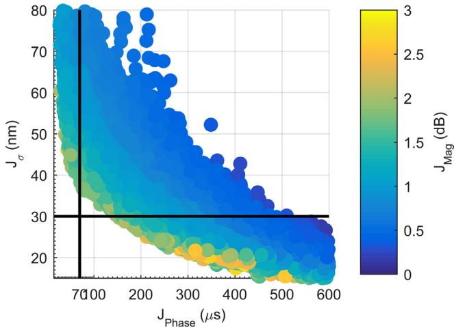
Fig. 14. Pareto front of H_{PZF} when \zeta = 1/\sqrt{2} .
