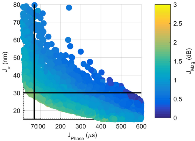
Fig. 15. Pareto front of H_{PZF} when 0 < \zeta \leq 1/\sqrt{2} .
