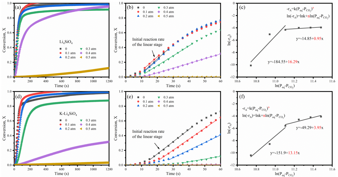
Figure 4. Regeneration plots under different CO_2 pressures at 700 °C, and the determination of reaction order by fitting plots for (a, b, c) Li_4SiO_4 and (d, e, f) K-Li_4SiO_4 .
