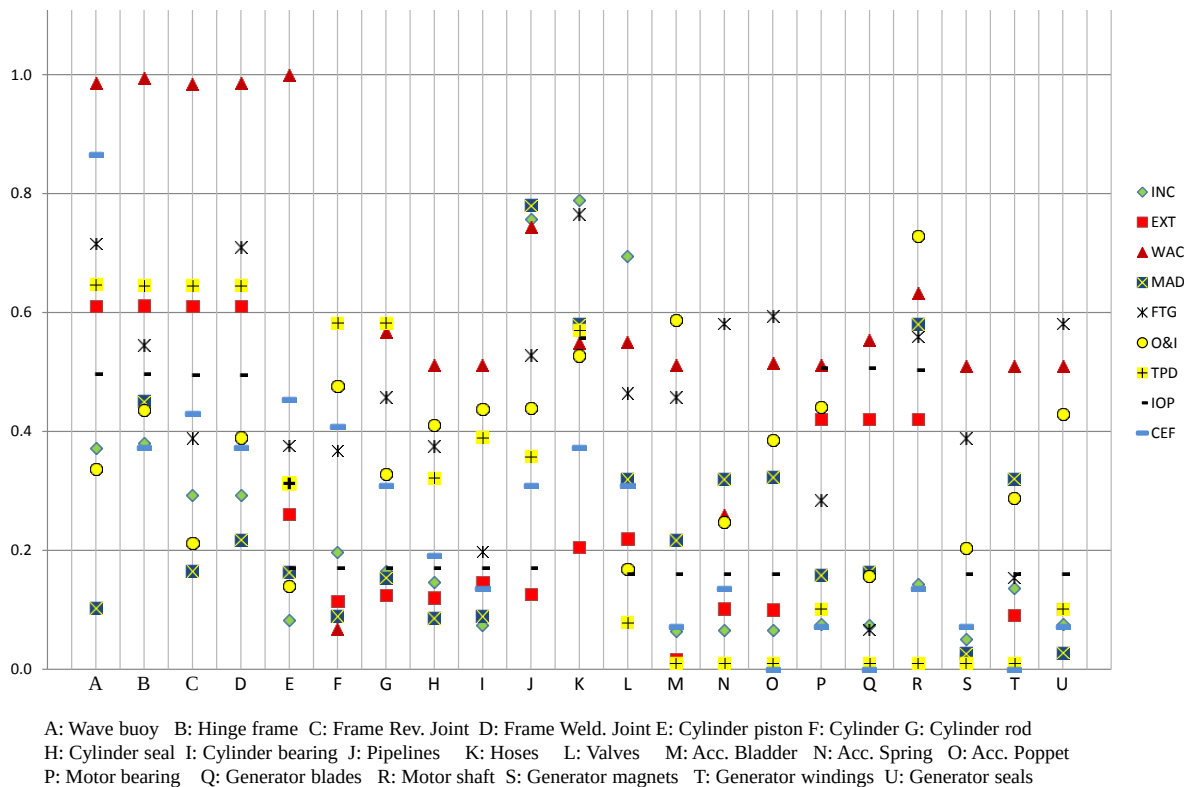
Figure 15: Contribution of failure modes towards components risk
