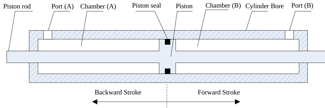
Figure 11 Longitudinal cross-section of double-rod double-acting cylinder
