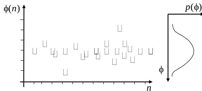
Figure 2 Frequency ( \phi ) and probability of frequency, p(\phi)
