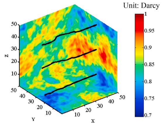
Fig. 18. Optimised horizontal laterals starting from various entrance points along the mainbore.
