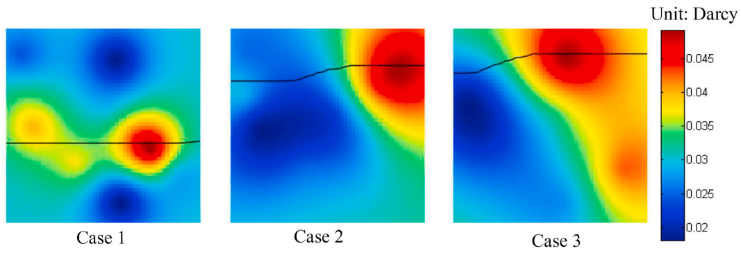
Fig. 12. Optimised well trajectories in heterogeneous reservoirs with different productivity potential distributions.
