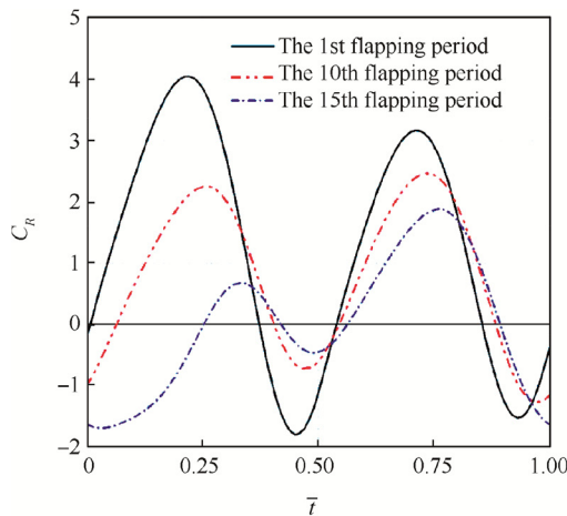
(a) Rotation moment coefficients
