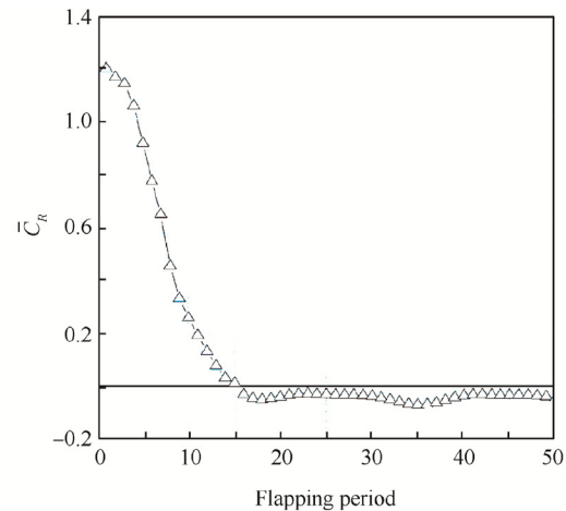
(b) Averaging rotation moment coefficients
