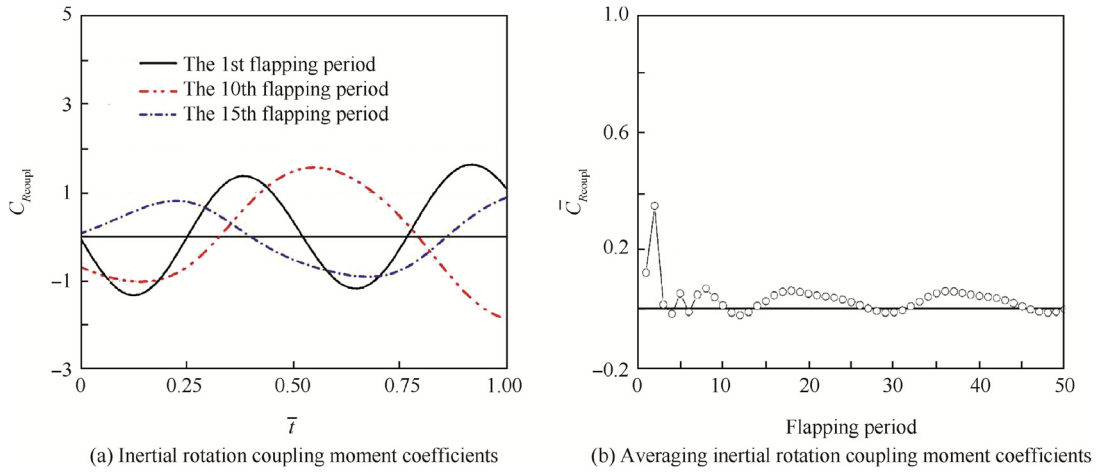
Fig. 7 Inertial rotation coupling moment coefficients C_{Rcoupl} varying in the 1st, 10th, 15th flapping period and averaging inertial rotation coupling moment coefficients \bar{C}_{Rcoupl} in each flapping period.
