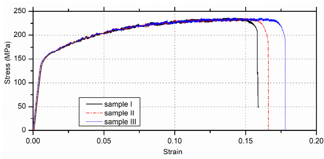
Fig. 2 Stress-strain curve of the base material AA5754 alloy (the test was repeated three times showing the peak deformation stress remains unchanged)
