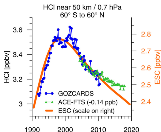
Fig. 1. Time series of near-global (60°S to 60°N) stratospheric hydrogen chloride (HCl) near 0.7 hPa (~50 km altitude). The plotted Global Ozone Chemistry And Related trace gas Data records for the Stratosphere (GOZCARDS) data are based on a combination of measurements from the Halogen Occultation Experiment (HALOE), Atmospheric Chemistry Experiment Fourier Transform Spectrometer (ACE-FTS) and Microwave Limb Sounder (MLS-Aura) satellite instruments (Froidevaux et al., 2015). ACE-FTS data are used to extend the time series, and are shifted to match the GOZCARDS data from 2002 to 2010. The thick orange line and the scale on the right give estimated effective stratospheric chlorine (ESC) for an age-of-air distribution with 5 years mean age and 2.5 years width (Newman et al., 2007). Updated from WMO (2011).
