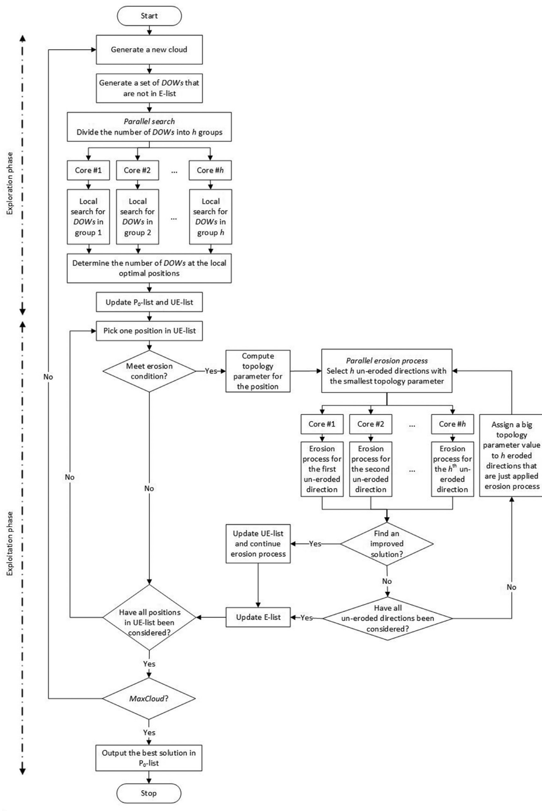
Fig. 6. A flowchart of the PWFA for the LARP.
