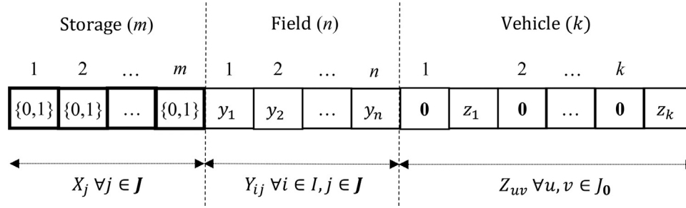
Fig. 3. A solution representation for the LARP.
