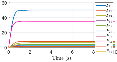
(b) Kernel matrix P(x_r) elements
