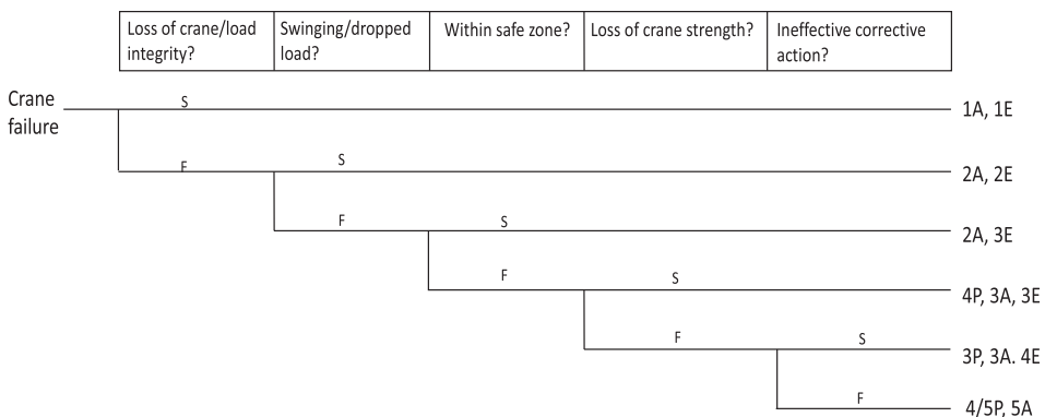
Figure 8. Crane failure event tree.
