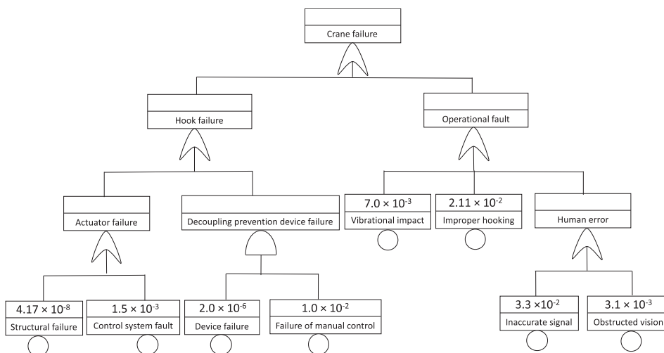
Figure 5. Fault tree diagram for crane failure event (intermediate event).
