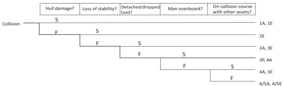
Figure 11. Collision consequence scenario 2.
