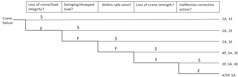
Figure 13. Crane failure consequence scenario 3.
