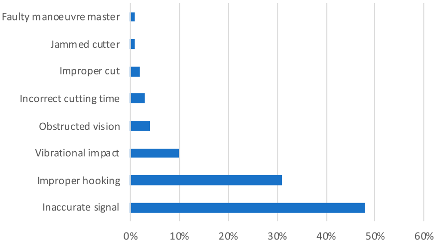
Figure 9. Importance ranking of basic events.
