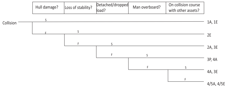
Figure 6. Collision event tree.
