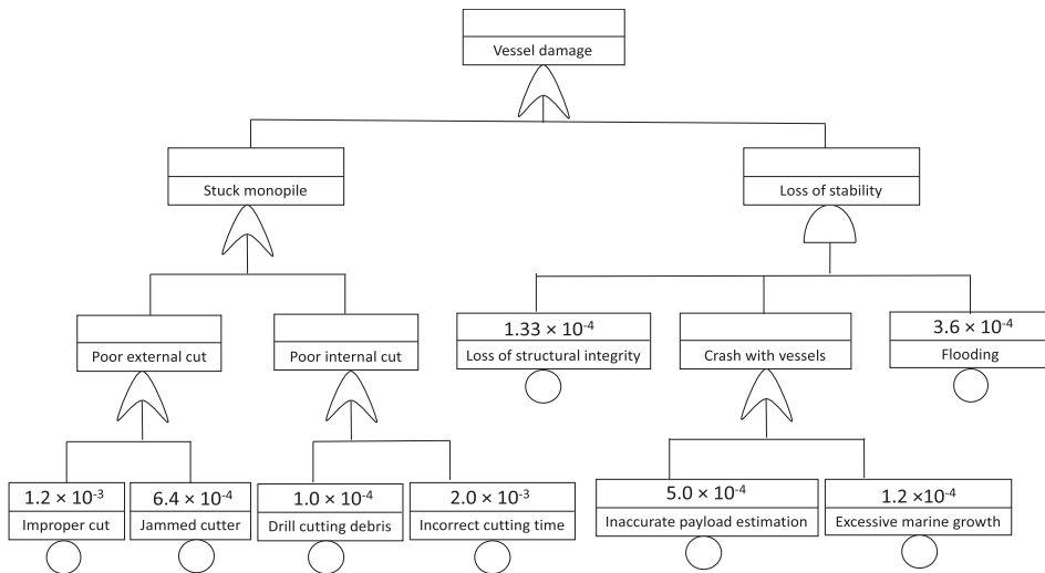
Figure 4. Fault tree diagram for vessel damage event (intermediate event).
