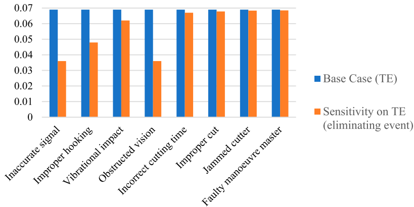
Figure 10. Sensitivity of basic events on top event.
