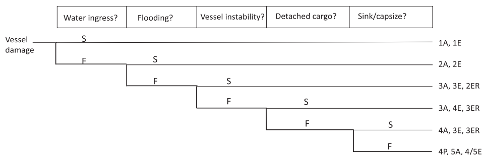
Figure 12. Vessel damage consequence scenario 3.
