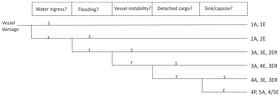
Figure 7. Vessel damage event tree.
