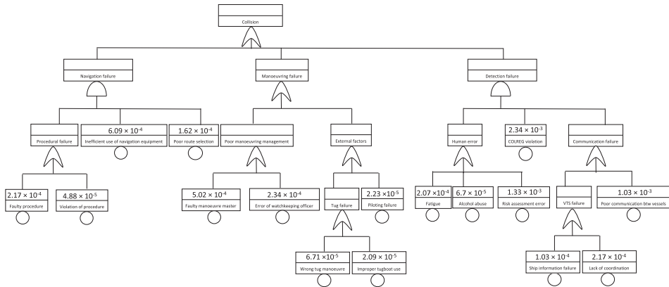
Figure 3. Fault tree diagram for collision event (intermediate event).
