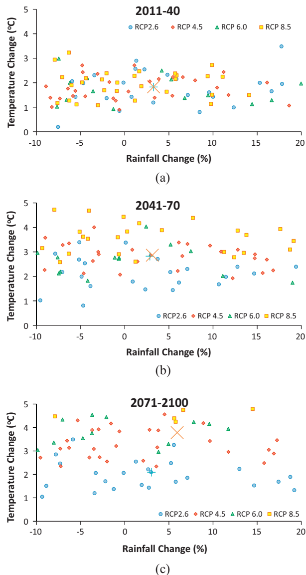
Fig. 6. Simulated changes in annual temperature and precipitation in the CMIP5-atlas ensemble relative to 1986–2005 (points show results of individual simulations; the crosses are the mean coordinates of the plotted points – see the text (Section 3.2) for further explanations).
