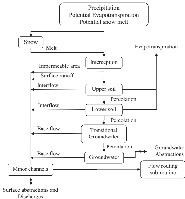
Fig. 3. HYSIM schematic.
