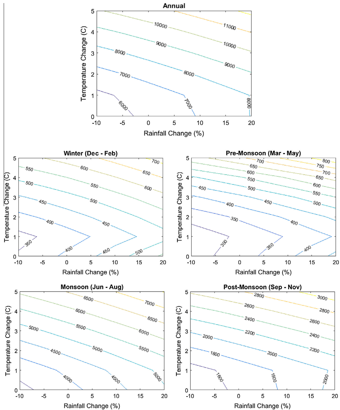
Fig. 8. Simulated mean annual and seasonal runoff at the Pong reservoir ( \text{Mm}^3 ).
