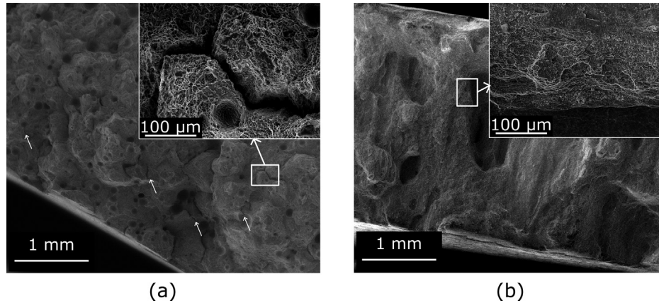
Fig. 8. Rupture surface of the 2024+2319 interfaces in (a) as-deposited and (b) inter-pass rolled conditions.
