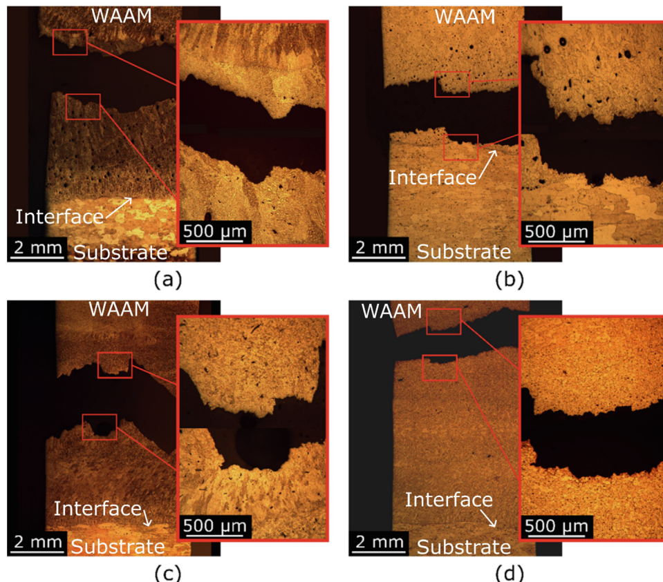
Fig. 3. Optical images of broken tensile specimens representative of the (a) as-deposited (un-rolled and non-heat treated), (b) heat treated, (c) inter-pass rolled, and (d) inter-pass rolled & heat treated.
