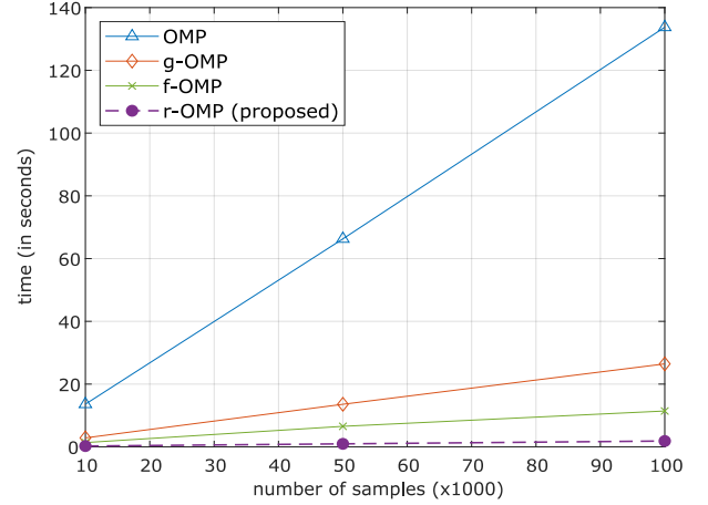
Fig. 1: Time taken by variants of OMP
