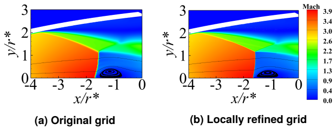
FIGURE 16: IMPACT OF GRID REFINEMENT ON RECIRCULATION REGION
