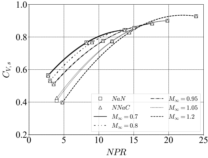
FIGURE 8: STANDARD VELOCITY COEFFICIENT VARIATION WITH NPR AND M_\infty FOR BOTH CONFIGURATIONS (CURVES DO NOT REPRESENT A TREND)
