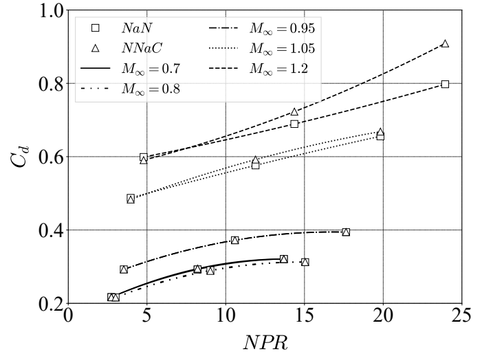
FIGURE 9: DRAG COEFFICIENT VARIATION WITH NPR AND M_\infty FOR BOTH CONFIGURATIONS (CURVES DO NOT REPRESENT A TREND)
