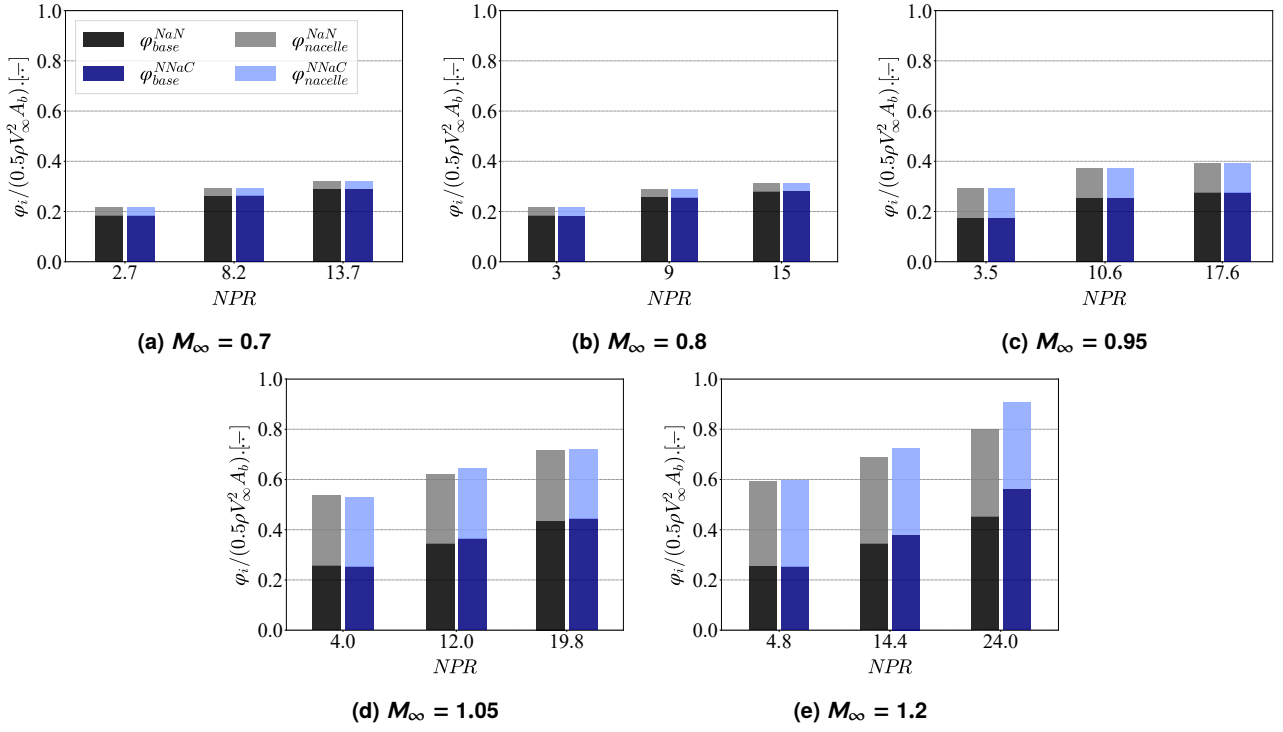
FIGURE 10: CONTRIBUTION OF CONSTITUENT ELEMENTS IN THE OVERALL DRAG COEFFICIENT ACROSS DESIGN SPACE
