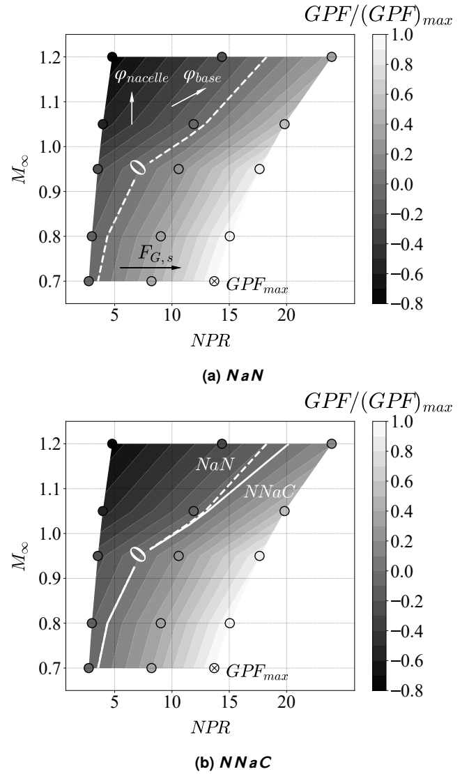
FIGURE 13: VARIATION OF GROSS PROPULSIVE FORCE WITH NPR AND M_\infty ACROSS DESIGN SPACE
