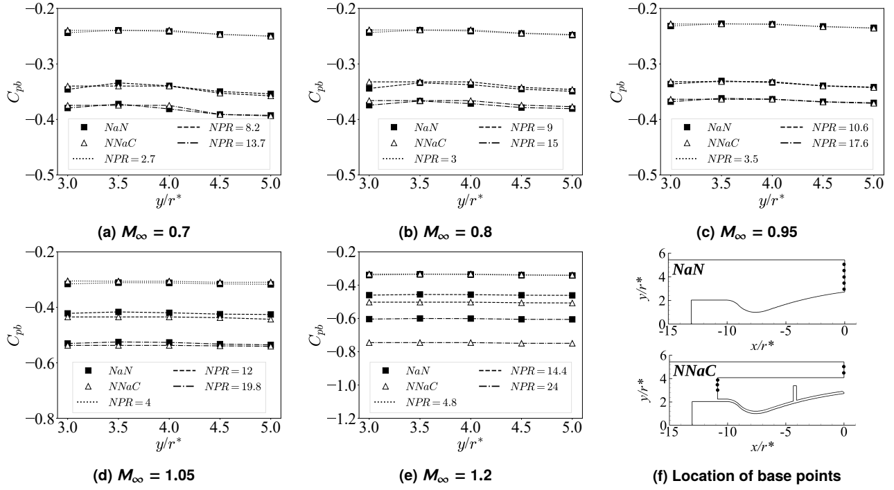
FIGURE 11: BASE PRESSURE COEFFICIENT ACROSS DESIGN SPACE FOR BOTH CONFIGURATIONS (LINES DO NOT REPRESENT A TREND)
