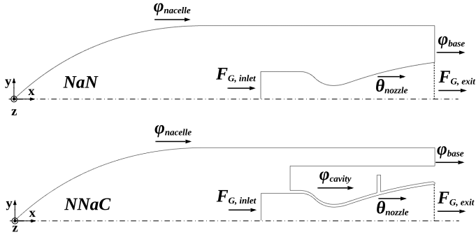
FIGURE 3: THRUST AND DRAG ACCOUNTING SYSTEM FOR THE INVESTIGATED CONFIGURATIONS
