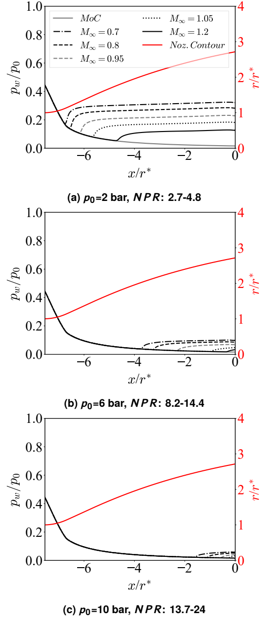
FIGURE 7: EVOLUTION OF NOZZLE WALL PRESSURE PROFILE WITH INCREASING M_\infty AND p_0 FOR NNaC
