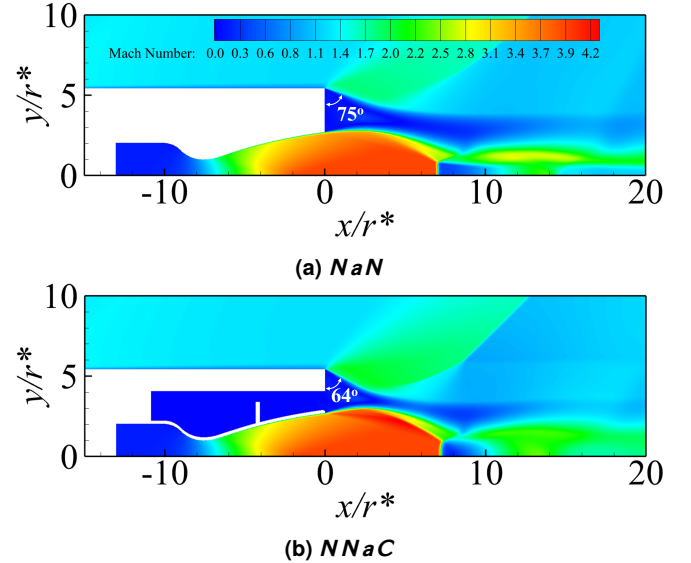
FIGURE 12: DISTRIBUTION OF MACH NUMBER AT CONDITIONS OF M_\infty=1.2 AND NPR_{max}=24
