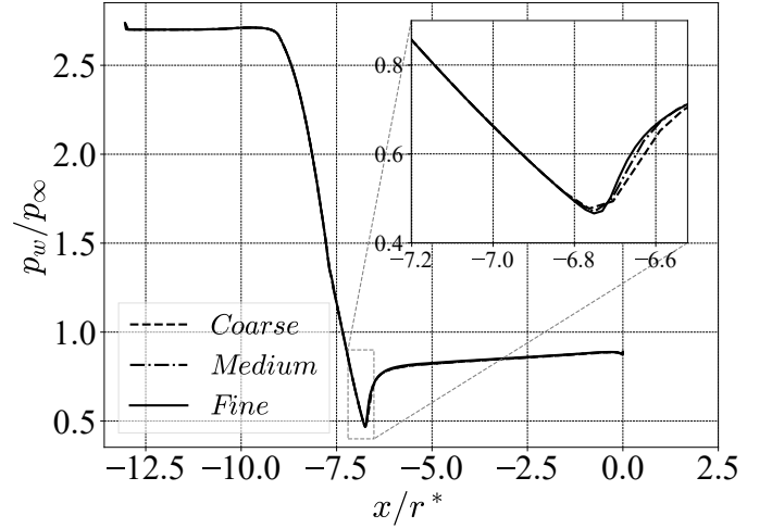
FIGURE 6: NOZZLE WALL PRESSURE PROFILE FOR THE THREE GRIDS AT NPR = 2.7 FOR NNaC
