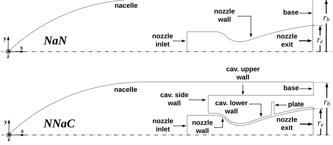
FIGURE 1: CONFIGURATIONS UNDER INVESTIGATION. NOZZLE AND NACELLE (TOP), NOZZLE, NACELLE AND CAVITY (BOTTOM)
