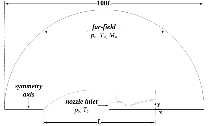
FIGURE 4: COMPUTATIONAL DOMAIN AND BOUNDARY CONDITIONS
