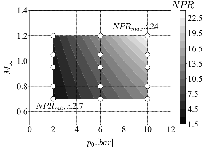
FIGURE 2: NPR VARIATION WITH M_\infty AND p_0 ; WHITE CIRCLES DENOTE THE TEST CASES
