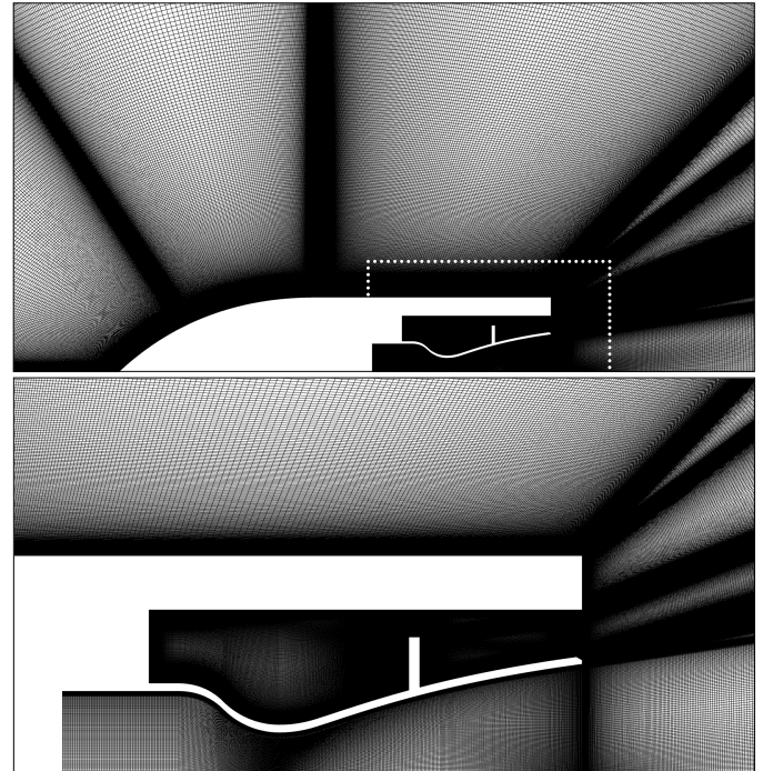
FIGURE 5: COMPUTATIONAL MESH (TOP) AND CLOSE-UP VIEW ON CAVITY AND NOZZLE REGIONS (BOTTOM)
