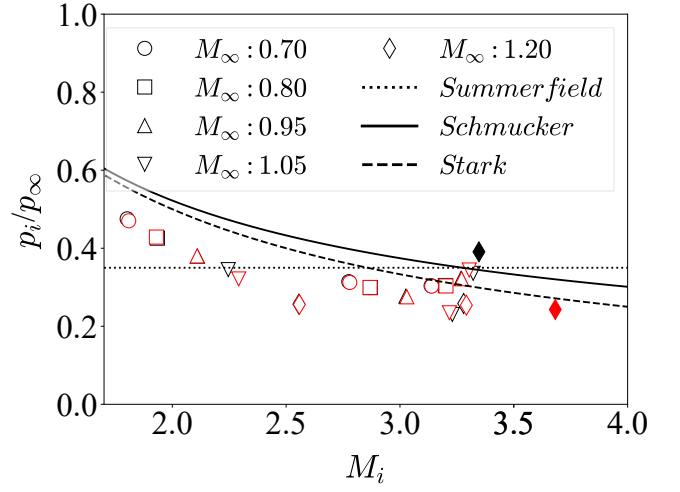
FIGURE 15: PRESSURE OF INCIPIENT SEPARATION AS A FUNCTION OF WALL MACH NUMBER
