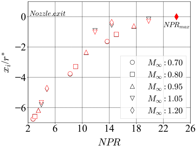
FIGURE 14: LOCATION OF INCIPIENT SEPARATION AS A FUNCTION OF NPR
