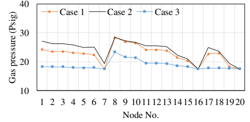
Fig. 10. Gas pressure for cases 1-3.
