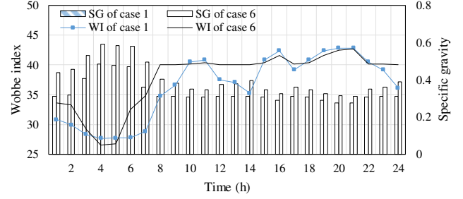
Fig. 9. Gas quality indices for cases 1 and 6.
