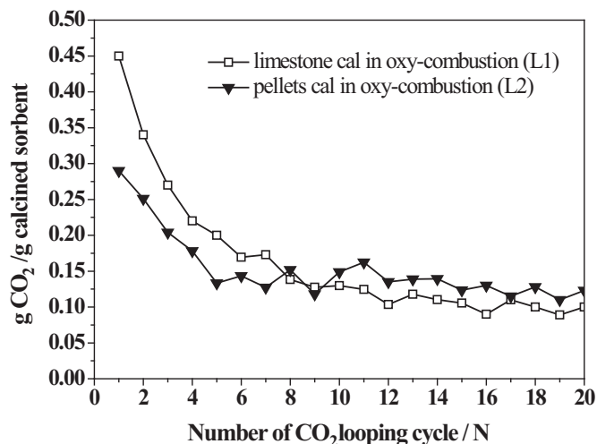
Fig. 4. \text{CO}_2 carrying capacity of sorbents versus looping cycle in fluidised bed.
