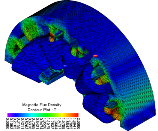
Fig. 6. Open-circuit magnetic flux density distributions of the proposed outer-rotor PMFS machine with meshes from 3-D FEA results.
