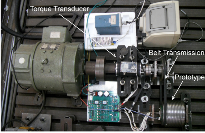
Fig. 13. Experimental setup for average torque measurements of the prototype machines.
