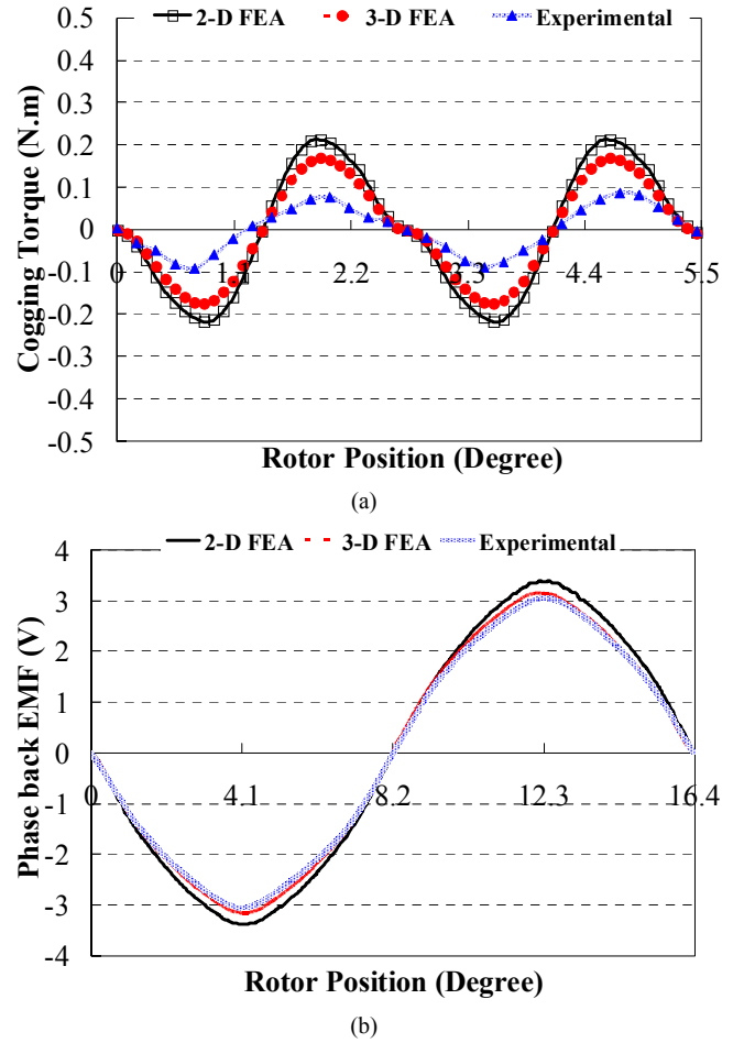
Fig. 12. Cogging torque and phase back EMF waveforms of the prototype machine from 2-D, 3-D FEA estimations and experimental measurement, (a) cogging torque profiles, (b) phase back EMF profiles.
