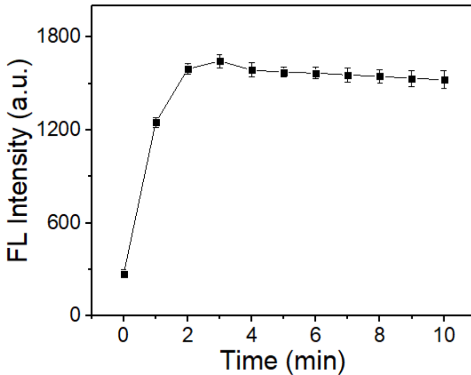
Fig. S14. Fluorescence intensity of GDYO-QDs / \text{Fe}^{3+} after reaction with AA ( 400 \mu\text{mol L}^{-1} ) for different times.
