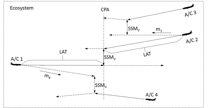
Figure 6. Ecosystem identification
