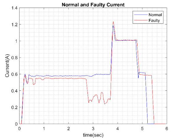
FIGURE 5. The normal and faulty current signals.
