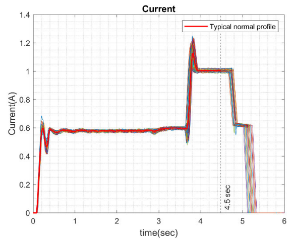
FIGURE 6. The typical normal current profile.
