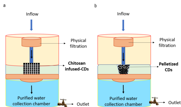
Figure 6. Lab-scale prototypes designed for assessing the water disinfection potential of CDs: (a) chitosan-infused CDs; (b) pelletized CDs.
