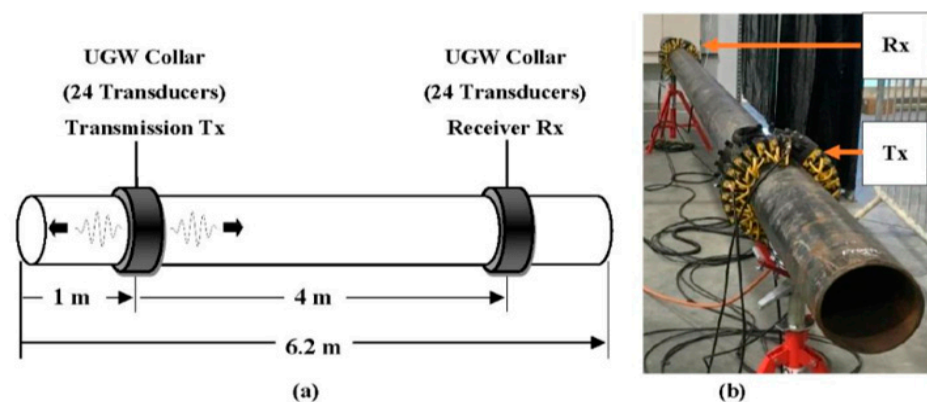
Figure 6. (a) Schematic and (b) setting-up of the UGW collar arrangement for pitch-catch configuration topology [89].
