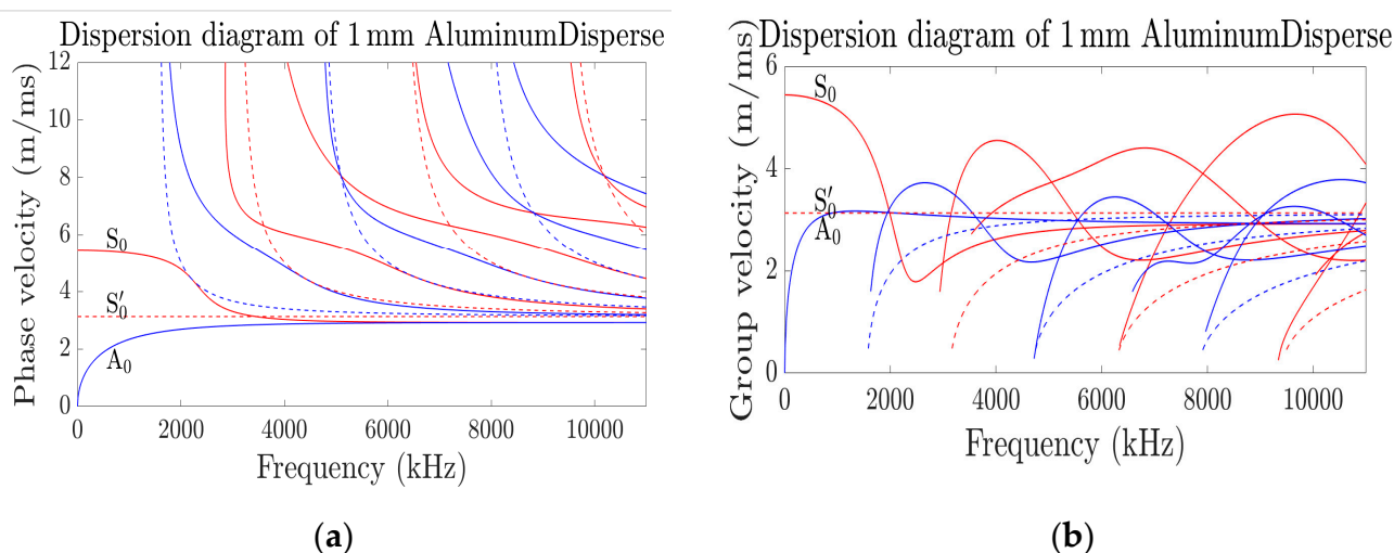
Figure 2. (a,b) Dispersive curve of 1 mm thickness of Al obtained using DC [77].
